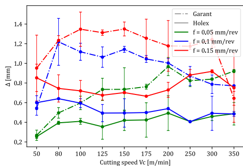
Fig. 4. Hole Entrance Eccentricity Measured on Aluminium 6082
