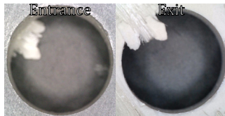
Fig. 8. Uncut fibers on GFRP plates
