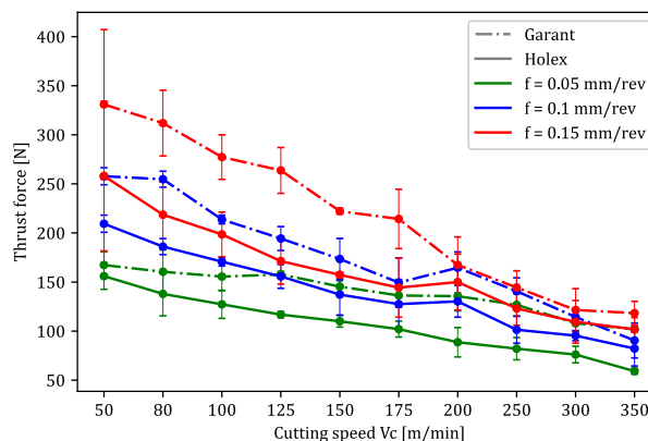
Fig. 2. Experimental thrust force (RMS values) during drilling on Aluminium 6082
