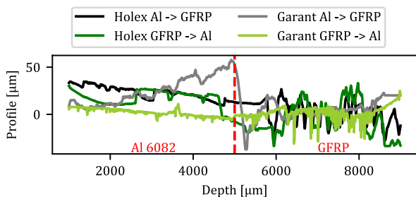
Fig. 10. 1D profile measurement on Al 6082 - GFRP stacks
