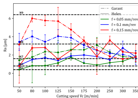
Fig. 6. Arithmetic roughness measurements on Aluminium 6082
