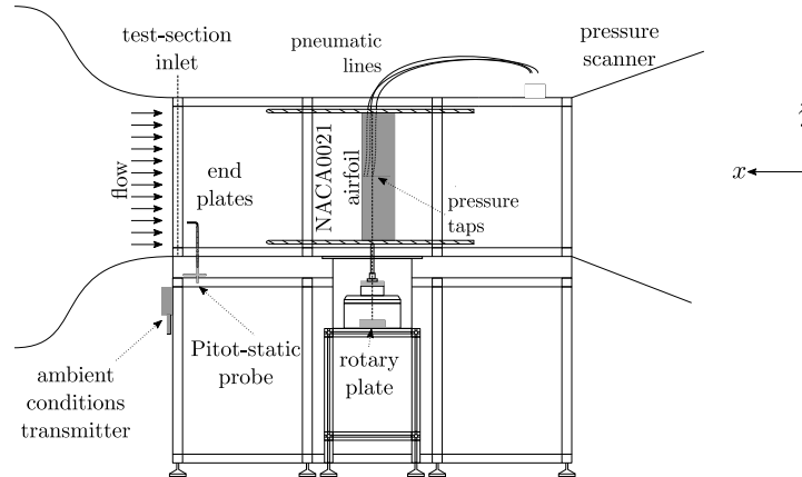
FIG. 1: Schematic illustration of the wind tunnel set-up for undertaking surface-pressure measurements upon an airfoil.
