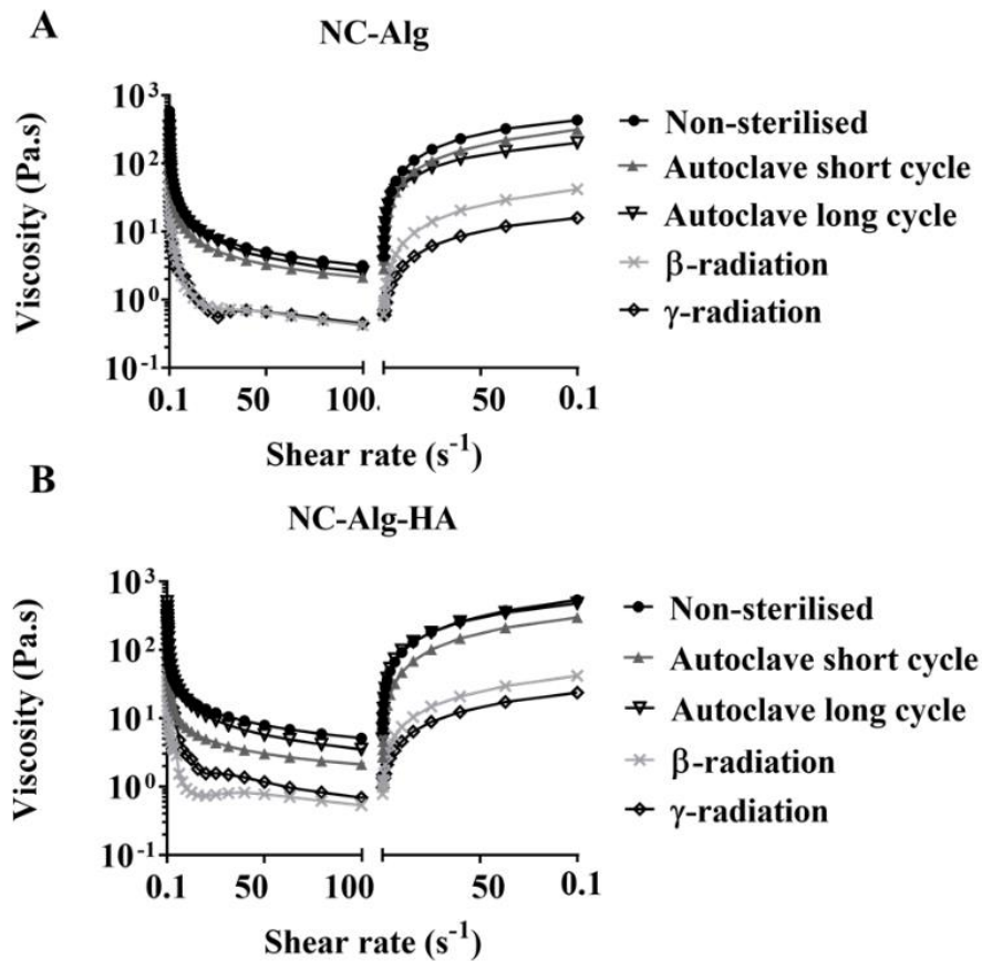
Figure 2. Effect of sterilisation methods on NC-Alg (A) and NC-Alg-HA (B) bioinks rheological properties. Viscosity values were measured before and after sterilisation by short and long cycle autoclaving, \beta -radiation and \gamma -radiation.
