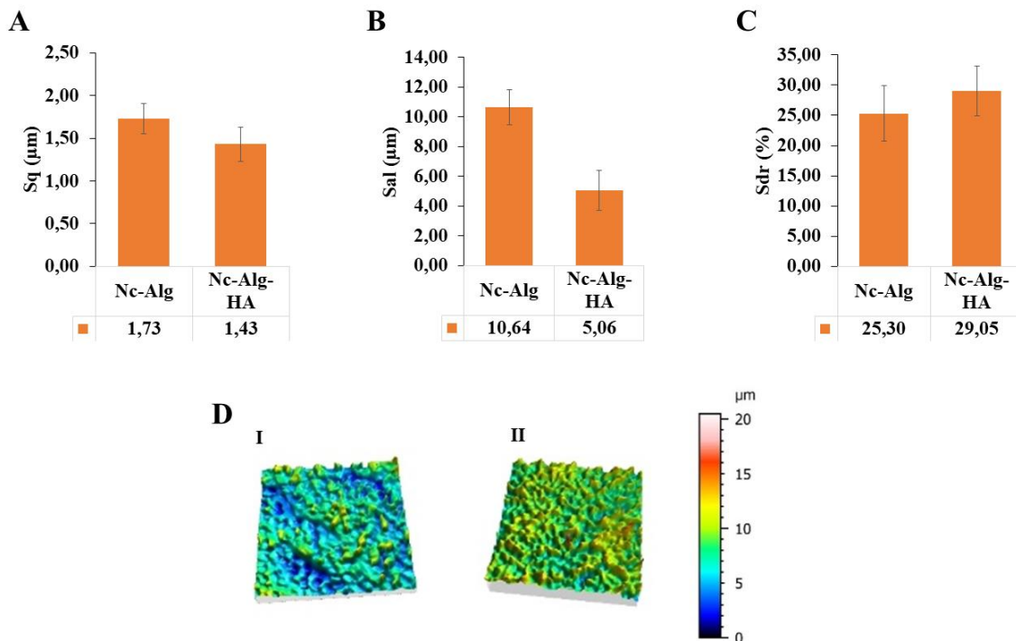
Figure 8 Surface and architectural structure study on NC-Alg and NC-Alg-HA scaffolds. A-C) 3D topographical parameters describing height ( S_q ), lateral ( S_{sal} ) and hybrid ( S_{dr} ) characteristics of the scaffolds. Values represent mean \pm SD. D) Representative axonometric projections of the topographical measurements of the NC-Alg (I) and NC-Alg-HA (II) scaffolds.
