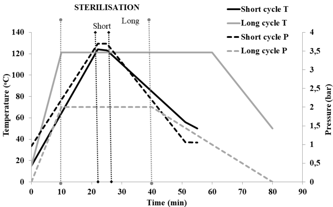
Figure 1. Comparison between short cycle and long cycle autoclaving procedures.
