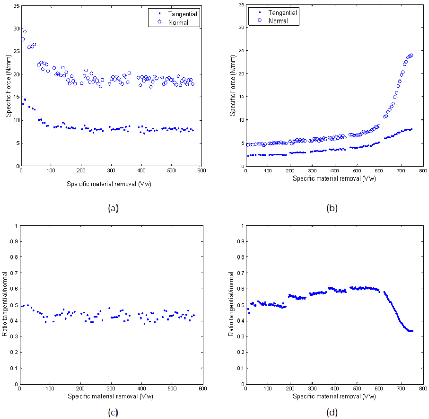
Fig. 5. Evolution of the forces with aggressive grinding parameters (a) and soft grinding parameters (b). Relationship between tangential and normal forces for aggressive grinding conditions (c) and soft grinding conditions (d).
