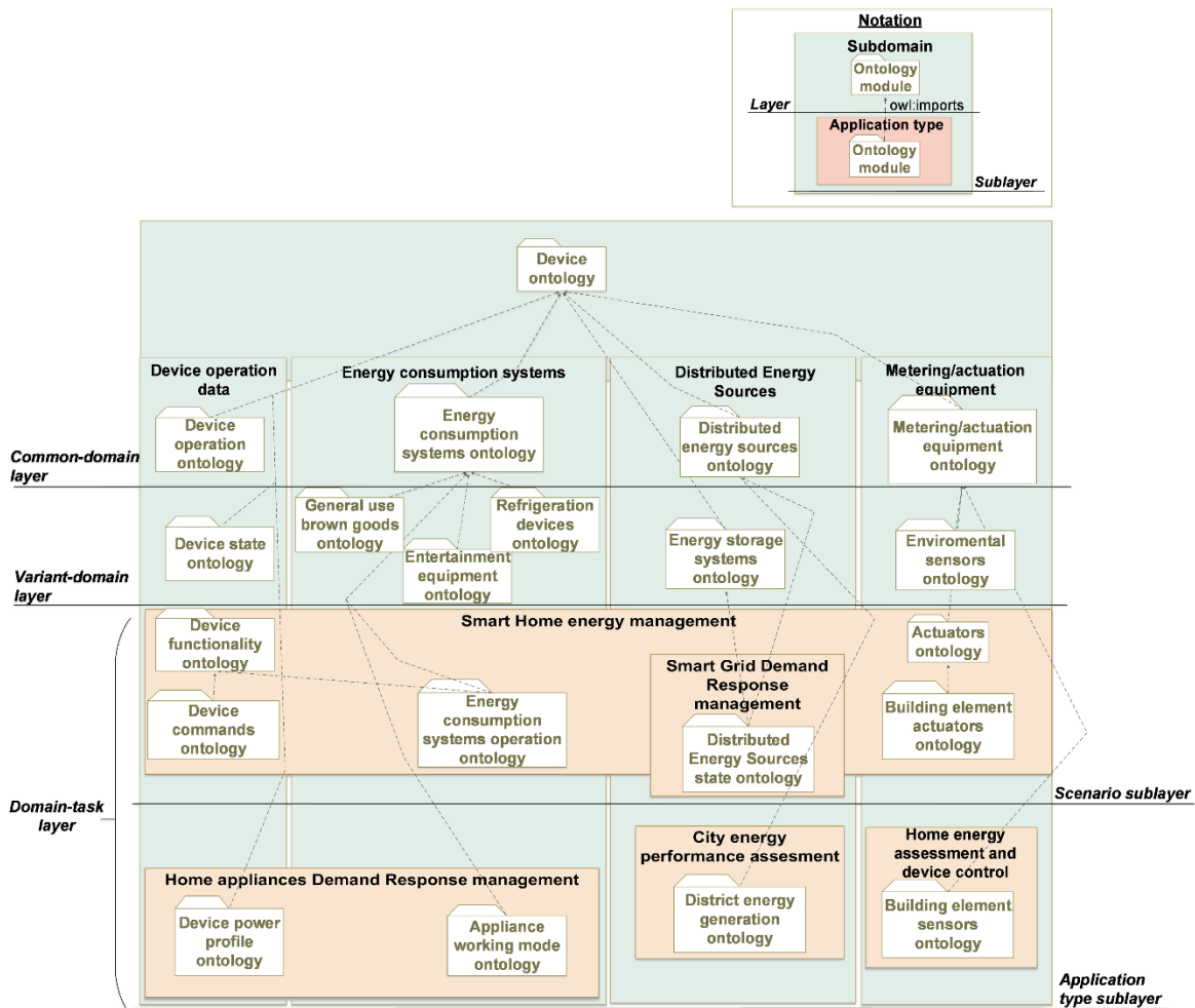
Figure 2: Structure of the DABGEO ontology (energy equipment domain)
