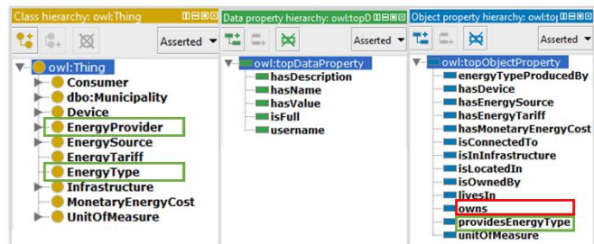
Figure 5: Class and property structure of the GEPSS ontology
