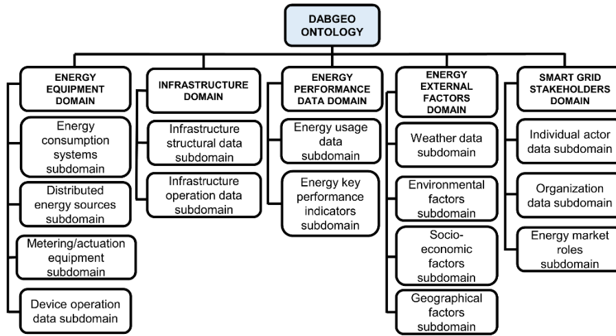
Figure 1: High-level structure of the DABGEO ontology
