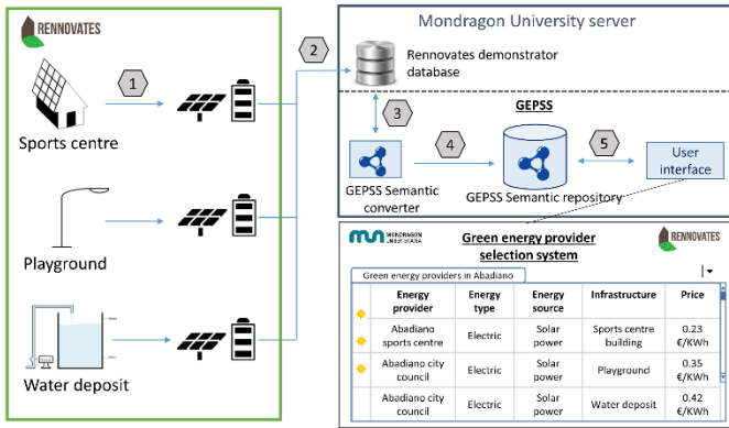
Figure 3: Architecture of the GEPSS
