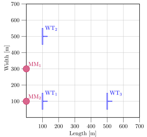
Fig. 6. Layout of the case study wind farm. The farm covers a 700 \times 700 \text{ m}^2 extension. The three wind turbines, indicated as WT_i , are 400 meters away in both directions (length and width). The measuring masts for wind monitoring are indicated as MM_j .
