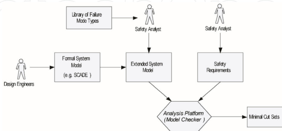
Figure 4. Principal components of failure injection approach [10].
