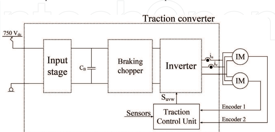
Figure 1. Tramway traction system schematics.
