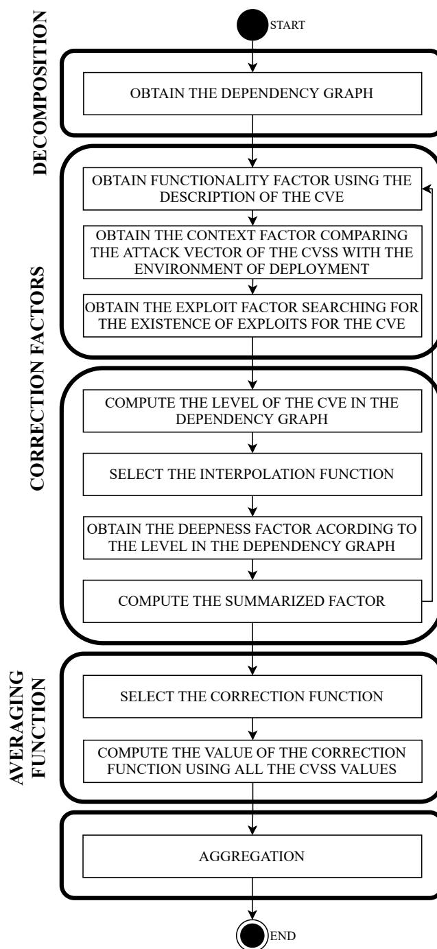
FIGURE 6.2: Flowchart showing the main steps of the aggregation algorithm for each CVSS.
