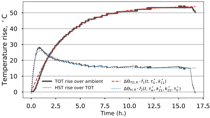
Fig. 7: Heat-run test based thermal parameter fitting.
