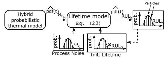
Fig. 5: Probabilistic lifetime modelling.
