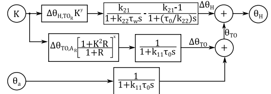
Fig. 1: Transient thermal model — adapted from [6].
