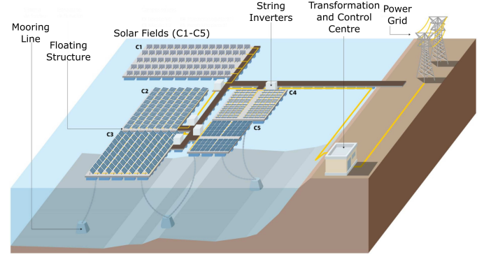
Fig. 6: Sierra Brava floating solar PV configuration.
