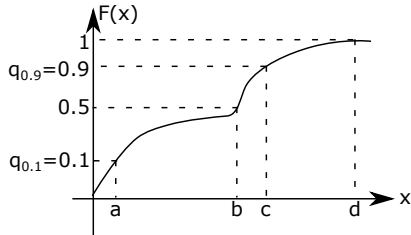
Fig. 4: Cumulative distribution function (CDF) and quantiles.
