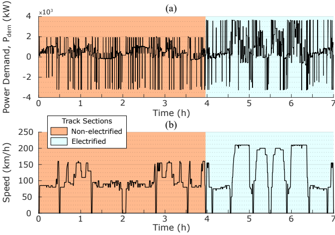
Fig. 2. Driving profile of "A Coruña - A Coruña" line: a) P_{dem} b) Speed.
