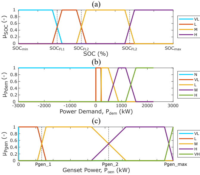
Fig. 6. Membership functions of Fuzzy Logic Strategy: a) LIB state of charge b) Power demand at DC bus c) Genset operation point. (N: Negative, VL: Very Low, L: Low, M: Middle, H: High, VH: Very High)
