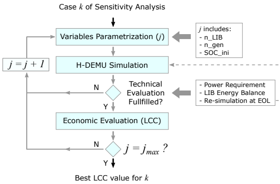
Fig. 9. Optimization by exhaustive search (DRB and DP strategies).
