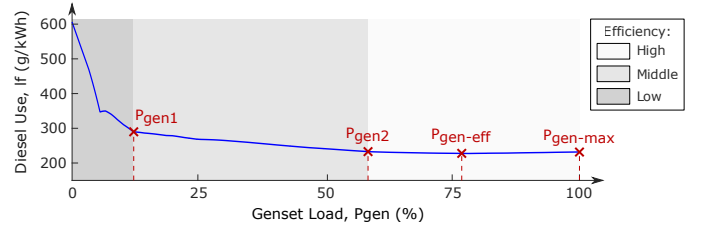
Fig. 3. Genset efficiency curve.
