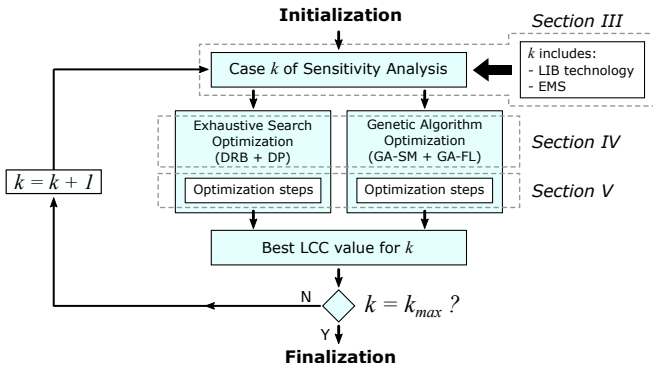
Fig. 8. Overview of sensitivity analysis, including two optimization approaches to obtain the LCC values: exhaustive search and genetic algorithms.
