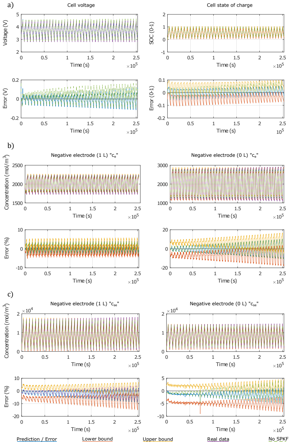
FIGURE 6. Cell voltage, SOC, c_e and c_{s,e} ROM and SPKF predictions and prediction errors for 40 cycles while aging..
