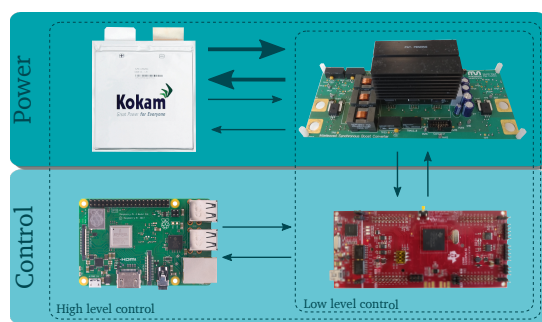
FIGURE 8. Validation platform general scheme. .
