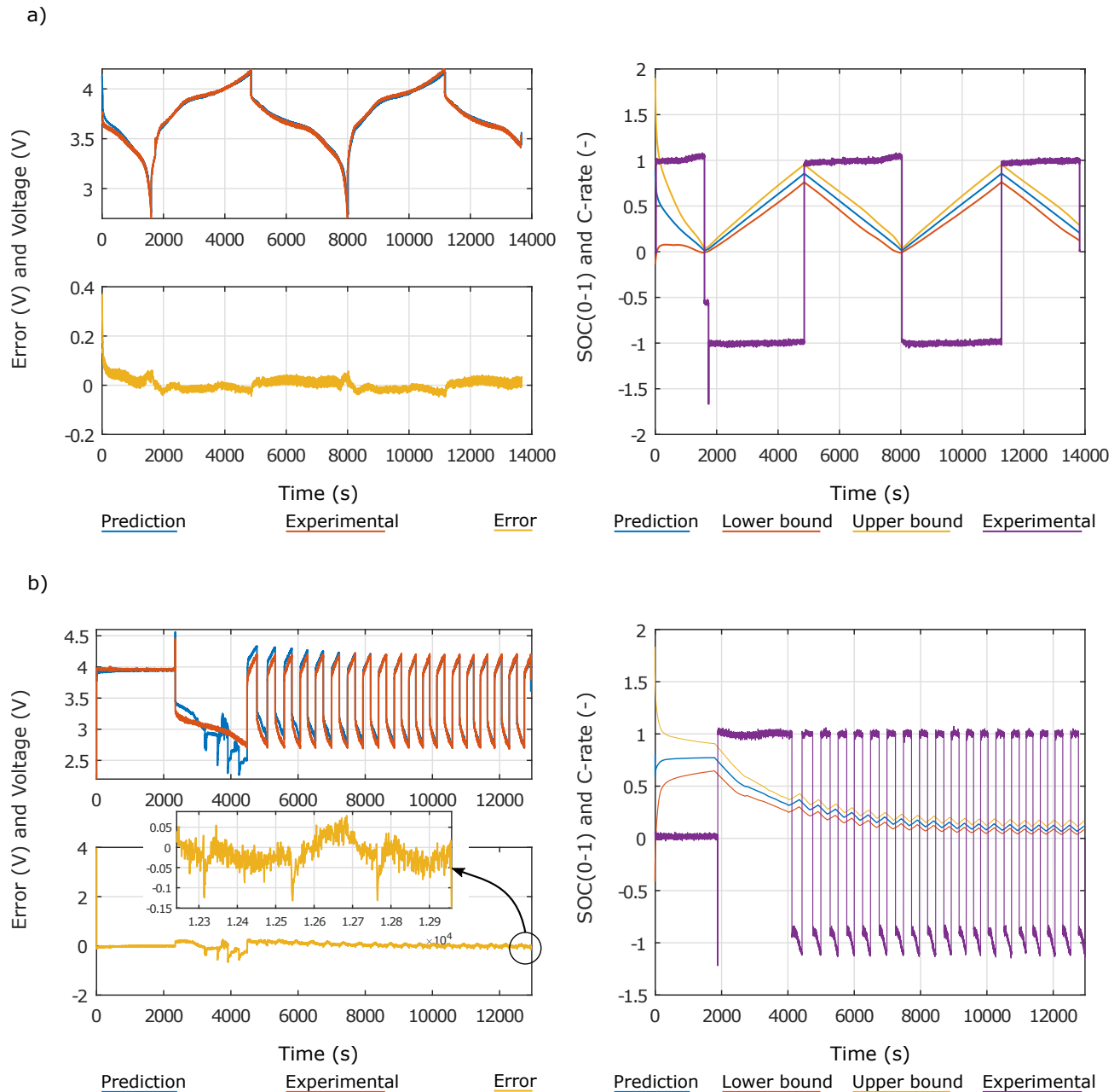
FIGURE 9. Experimental validation waveforms at room temperature (a) and at -10 °C (b).
