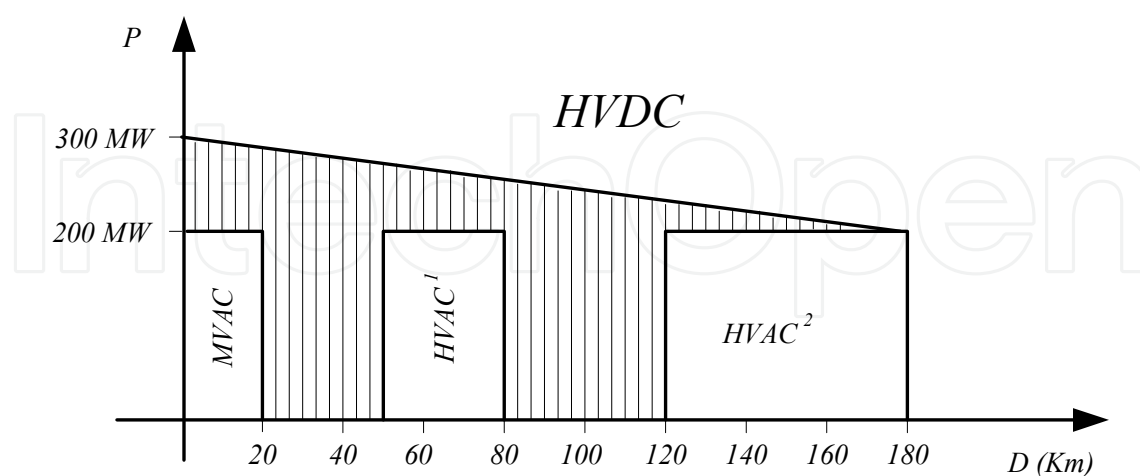
Figure 3.9 Optimum configuration depending on distance to shore and rated power: (1) With reactive compensation at both ends, (2) With reactive compensation at both ends and another one in the middle of the submarine cable.
