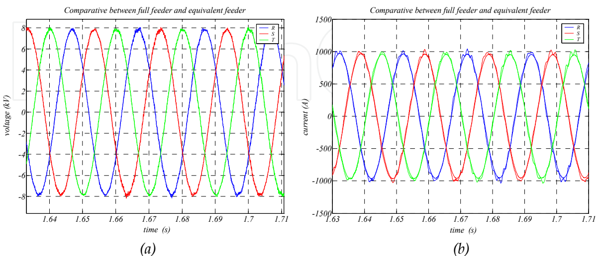
Figure F.5 Comparison of the equivalent wind turbine and the full feeder for a three-phase fault, the voltage (a) and current (b) at the PCC during the maintenance of the fault.
