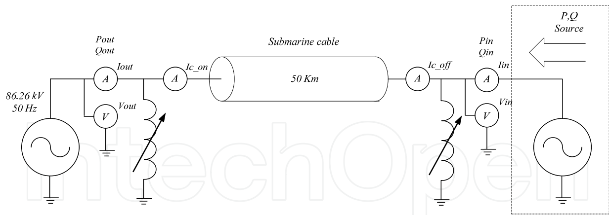
Figure 4.43 Diagram of the third simulation scenario, submarine cable with the injection of the inductive reactive power at both ends depending on the requirements.
