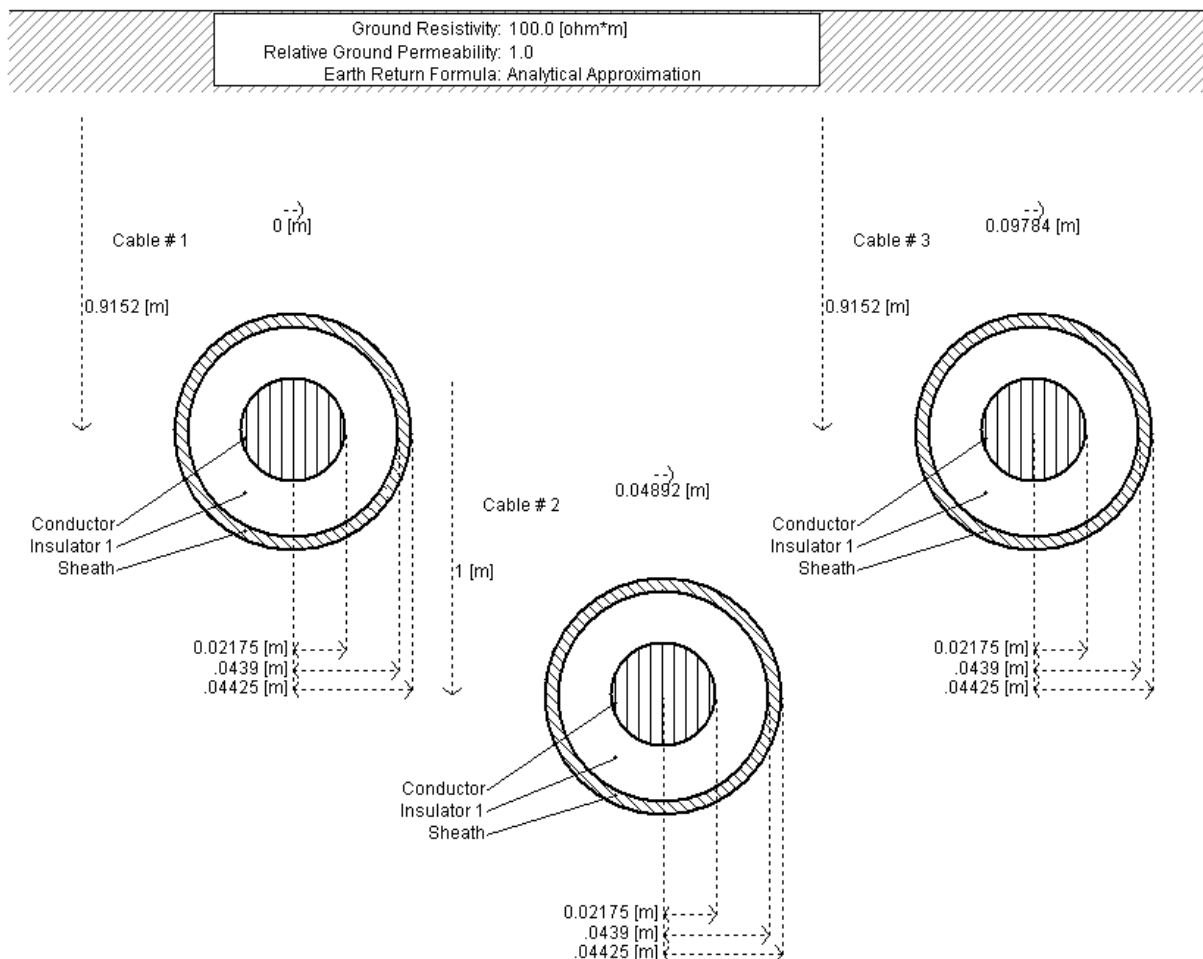
Figure 4.33 Graphic representation in PSCAD of the three-phase cable.
