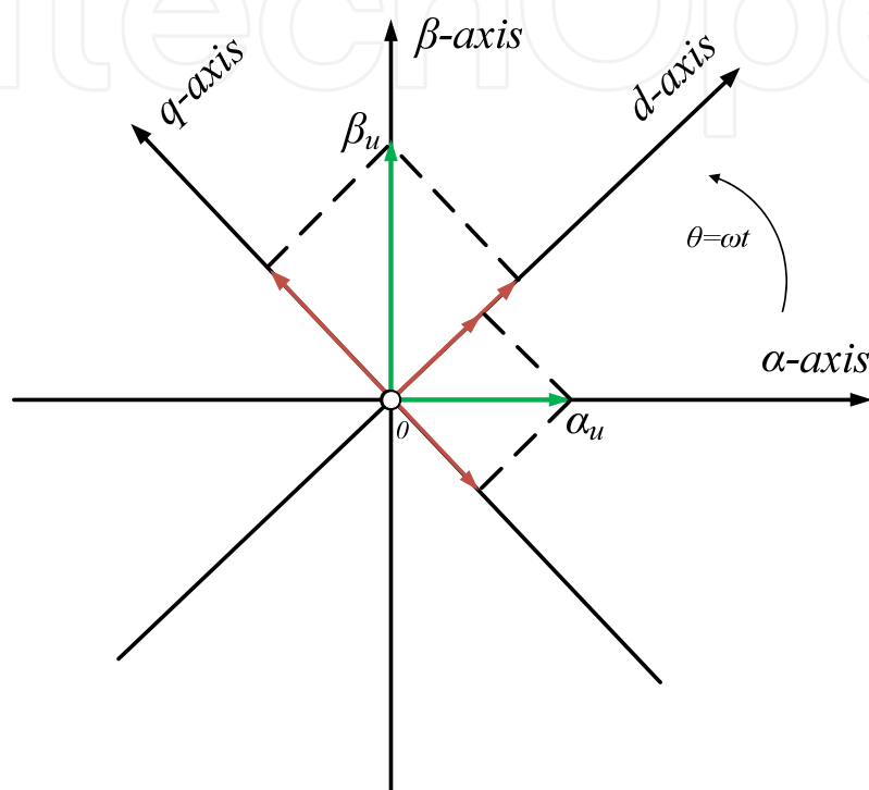
Figure D.2 Vector representation of the \alpha\beta to dq transform.
