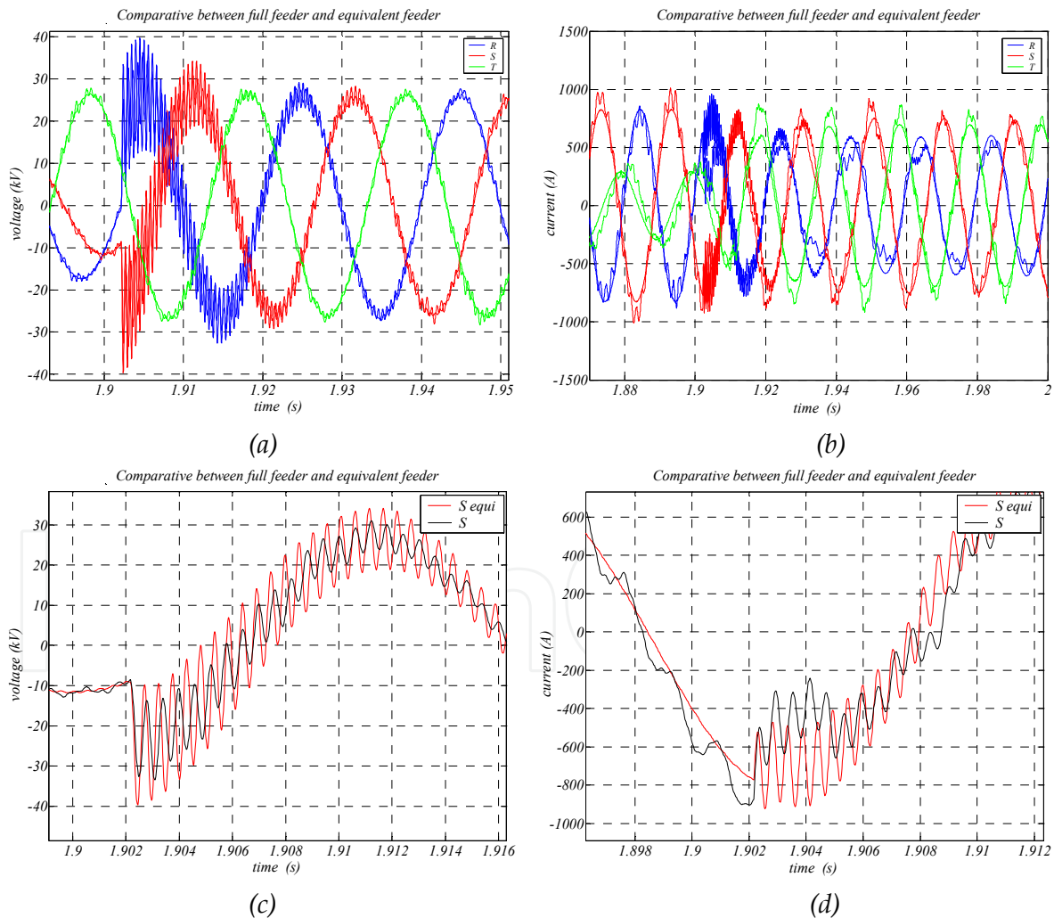
Figure F.11 Comparison of the equivalent wind turbine and the full feeder for a two-phase fault, the voltage (a) and current (b) at the PCC when the clearance of the fault occurs. (c)-(d) the voltage and current at the clearance of the fault mono-phase and more detailed, (red, equivalent feeder).
