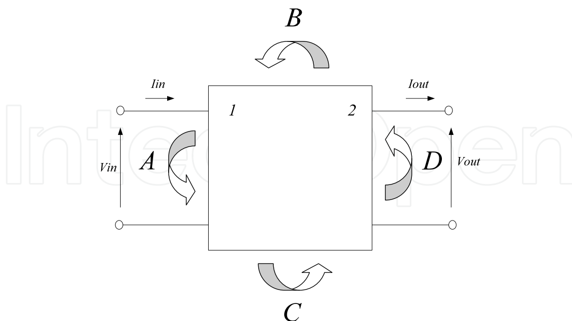
Figure 4.16 Two port system or quadripole oriented to a transmission line in phasor domain.
