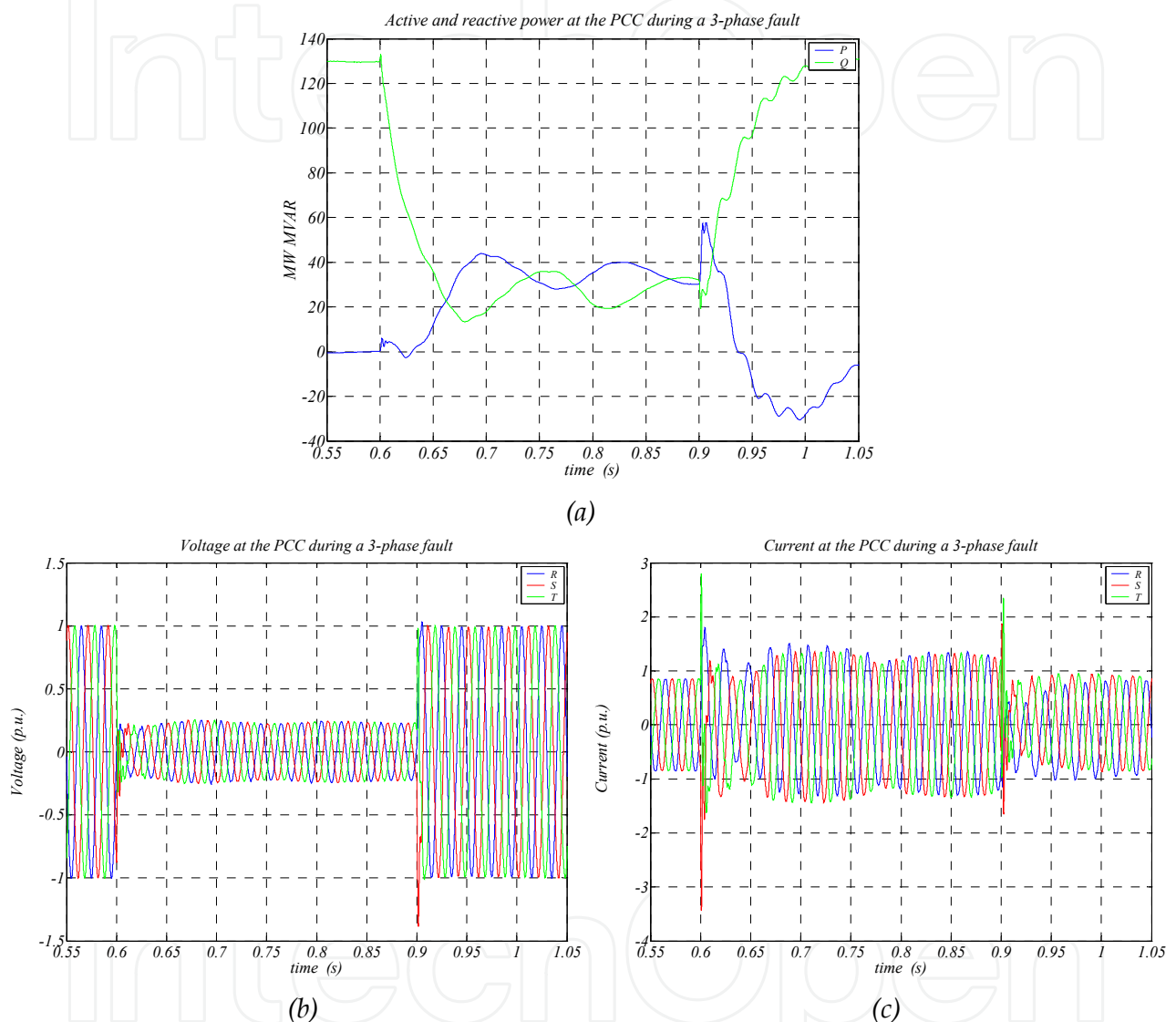
Figure 7.22 Current, voltage and active /reactive power at the PCC for the considered simulation scenario upon 3-phase 80% dip.
