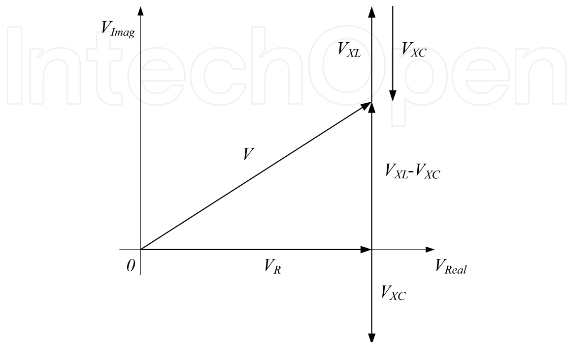
Figure E.4 Diagram of the voltages of the RLC branch.
