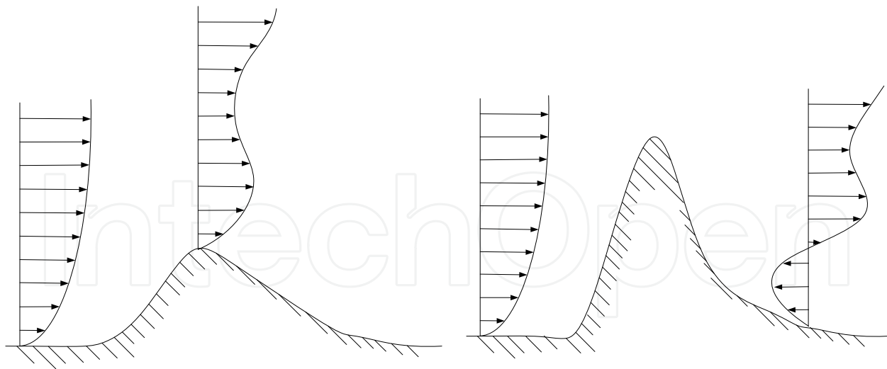
Figure 2.4 Illustration of the wind speed variation due to the obstacles in the earth surface.
