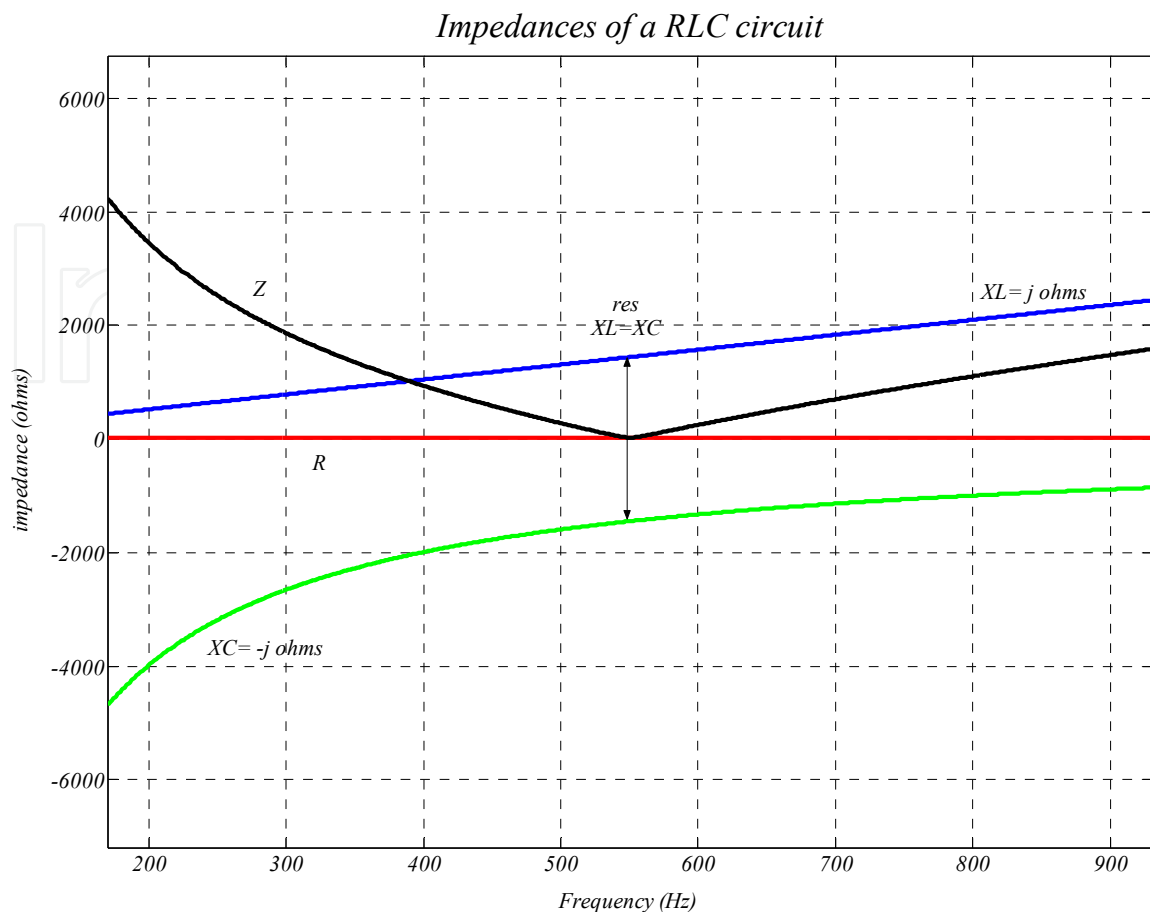
Figure E.5 Impedance of each component of the RLC branch depending on the frequency.
