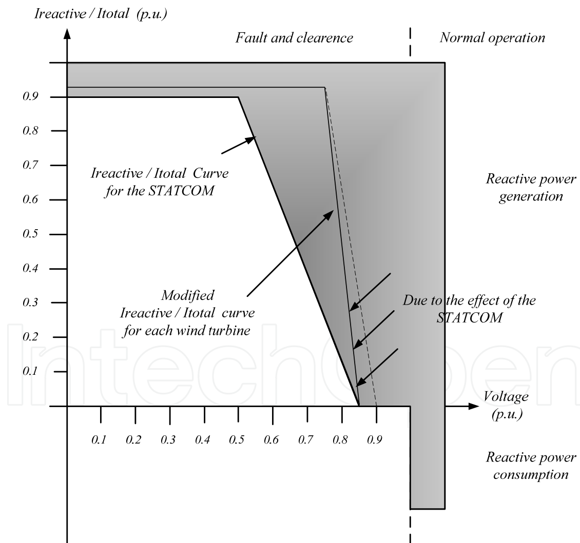
Figure 7.33 Proposed Ireactive / Itotal curve depending on the voltage to fulfill the REE requirements at the PCC.
