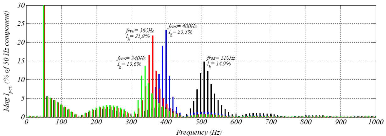
Figure 6.9 Frequency response of the transmission system varying the short circuit impedance from: 2 % (black), 5 % (blue), 8 % (green) and 11 % (red).
