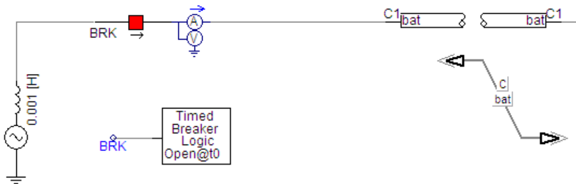
Figure 4.30 Simulation scenario in PSCAD for the Bergeron's travelling wave model.
