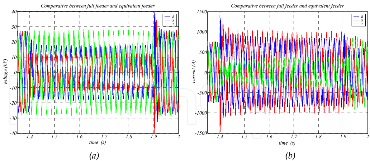
Figure F.8 Comparison of the equivalent wind turbine and the full feeder for a two-phase fault, the evolution of the voltage (a) and current (b) at the PCC during the fault and the clearance.
