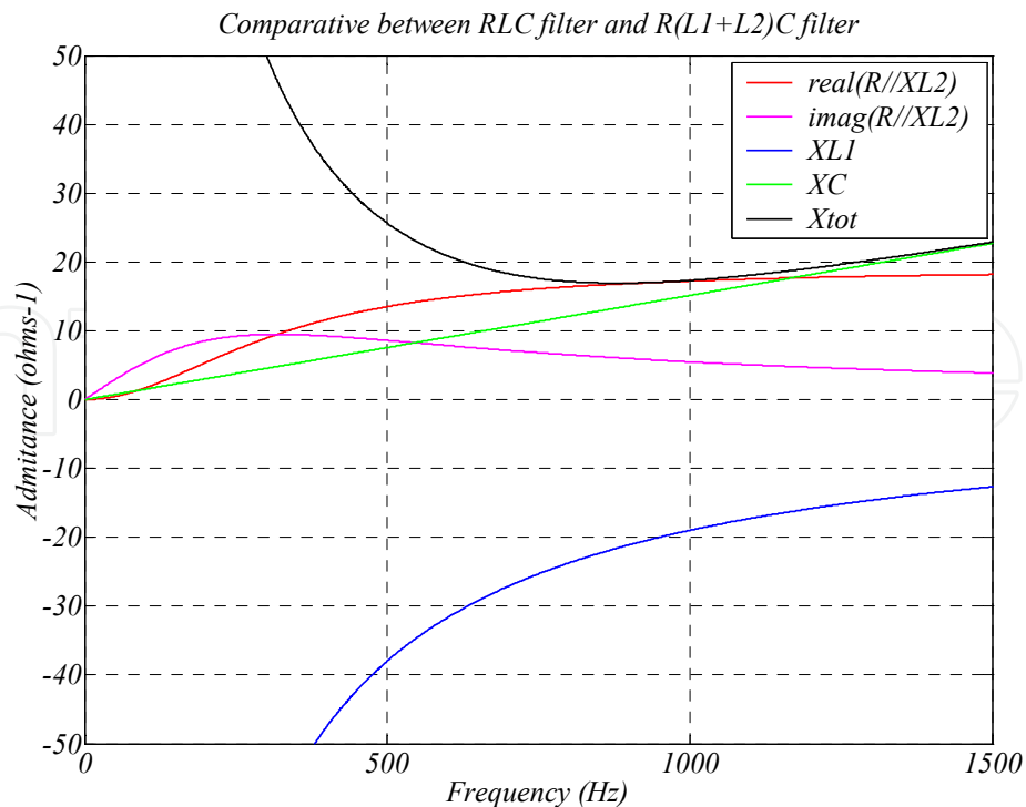
Figure E.11 Impedance of the (R+L)LC branch depending on the frequency and for each component.
