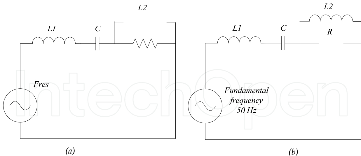
Figure E.8 Equivalent (R+L)LC circuit approximation depending on the frequency, (a) At resonance frequency and (b) at fundamental frequency.
