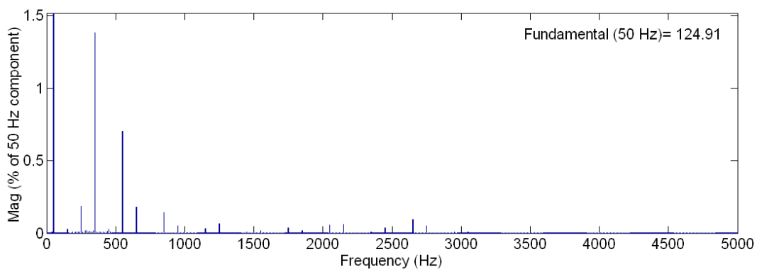
Figure 6.26 FFT of the voltage at the PCC for the base scenario while is transmitting / generating the nominal active power
