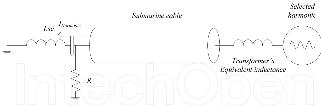
Figure E.2 Transmission system with a RLC filter at the resonance frequency of the filter.
