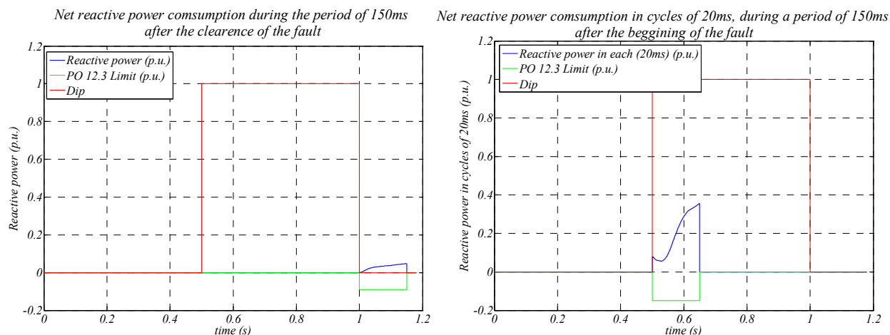
Figure 7.37 Summarized graphical results of a 2 nd category fault for the test defined in the PVVC, reactive power consumption in C zone and A zone.
