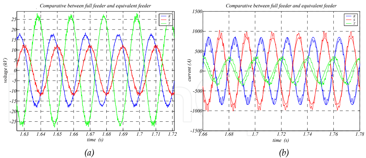
Figure F.10 Comparison of the equivalent wind turbine and the full feeder for a two-phase fault, the voltage (a) and current (b) at the PCC during the maintenance of the fault.
