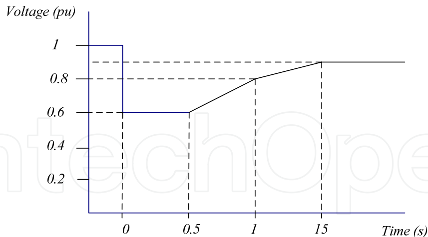
Figure C.2 Voltage / time curve admitted at the PCC for two-phase ungrounded faults
