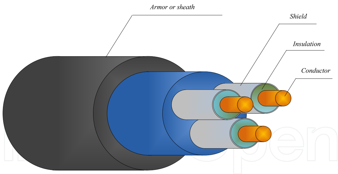
Figure 4.1 Generic representation of a electric power cable.
