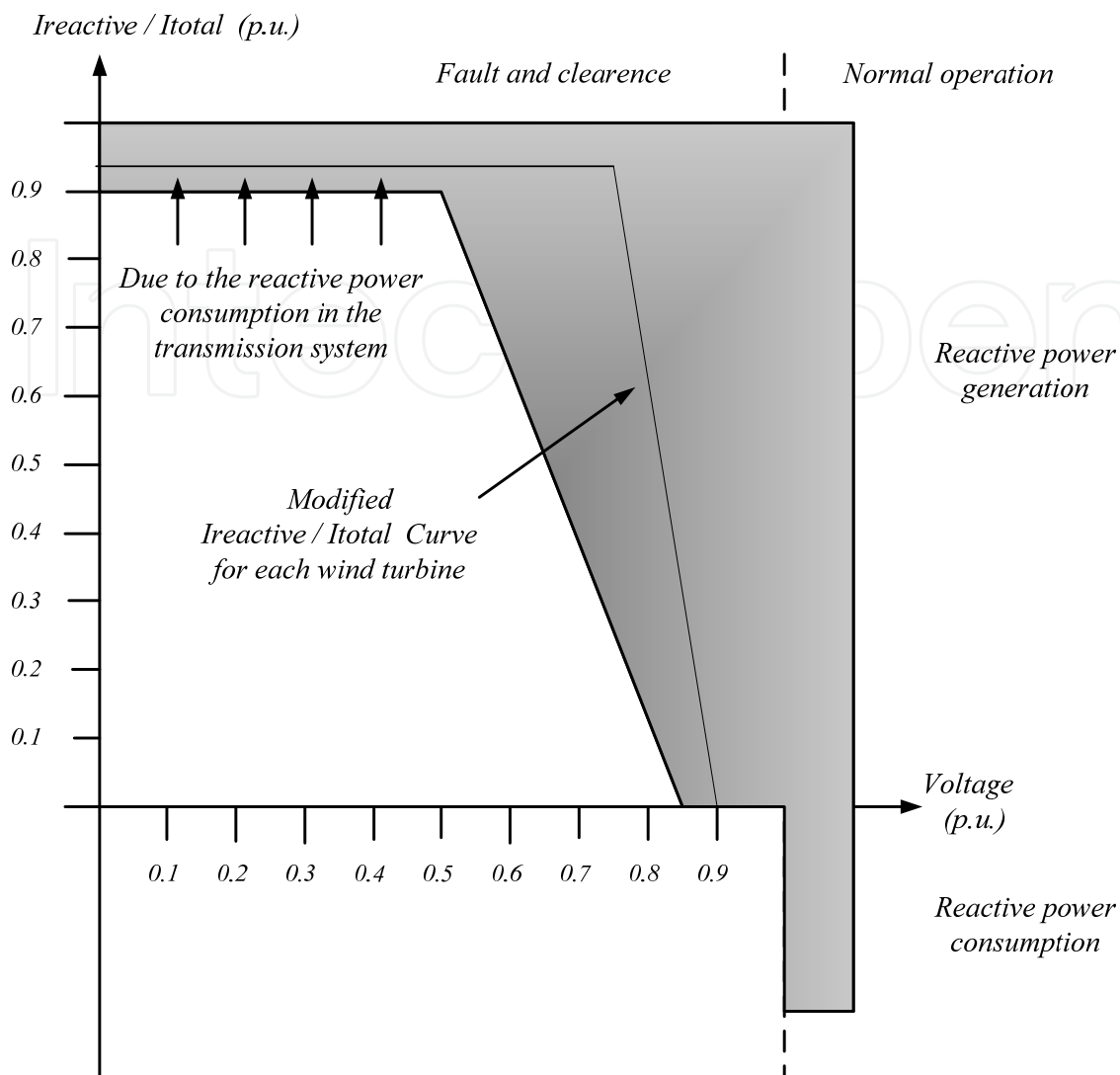
Figure 7.32 Modified Ireactive / Itotal curve depending on the voltage to fulfill the REE requirements at the PCC by reducing the injected active power during faults.
