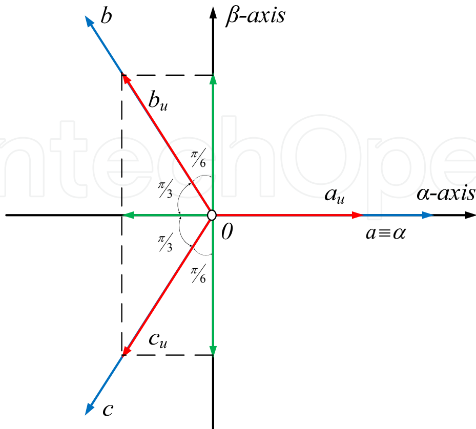
Figure D.1 Vector representation of the abc to a\beta transform.
