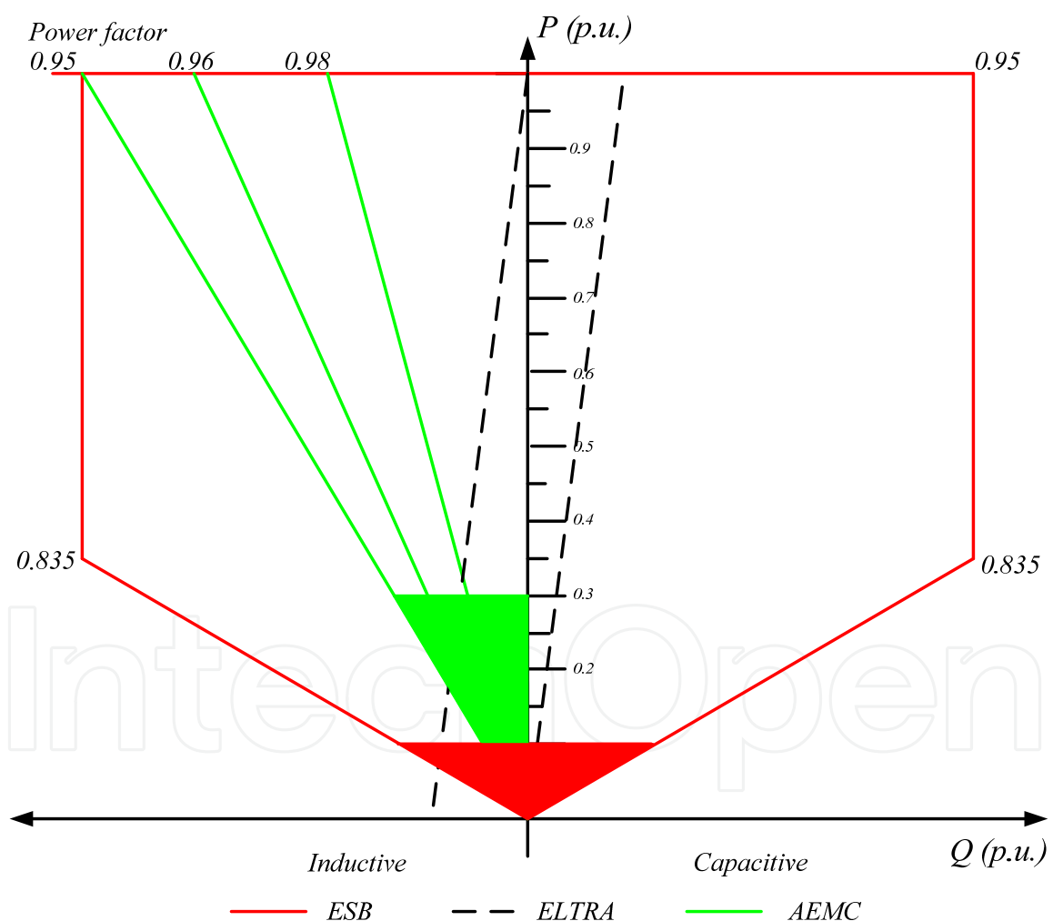
Figure B.1 Power factor requirements at the PCC for several international grid codes.
