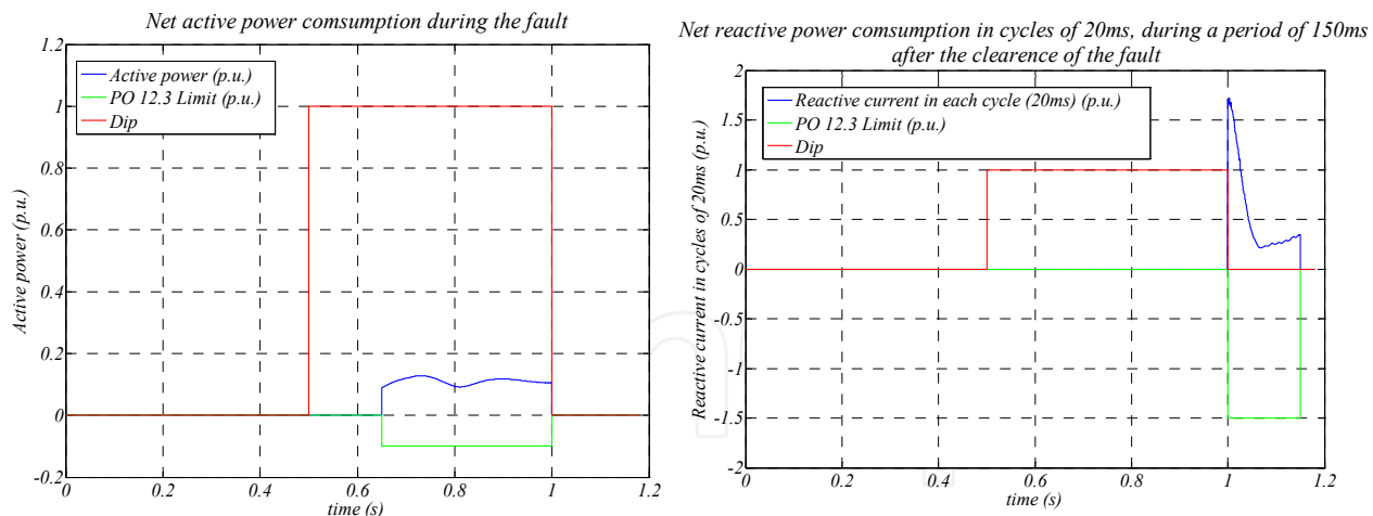
Figure 7.36 Summarized graphical results of a 2 nd category fault for the test defined in the PVVC, reactive current and power consumption in B zone and reactive current consumption in C zone.
