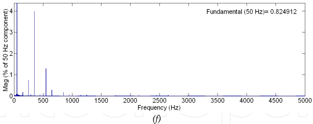
Figure 6.25 FFT of the current at the PCC for the base scenario while is transmitting / generating the nominal active power.
