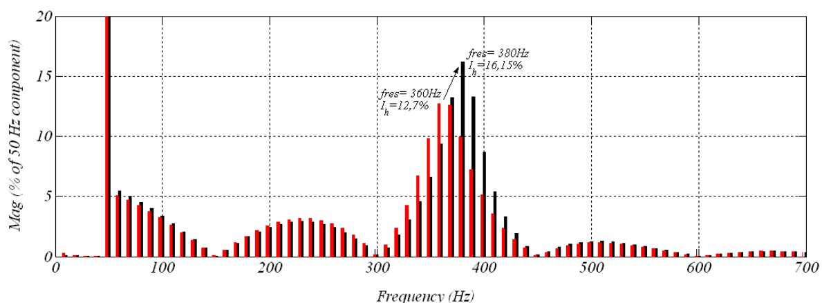
Figure 6.15 Harmonic currents at the PCC depending on the location of the harmonic voltage source inside the inter turbine grid. Substituting the 30 th wind turbine (red) and substituting the 25 th wind turbine (black).
