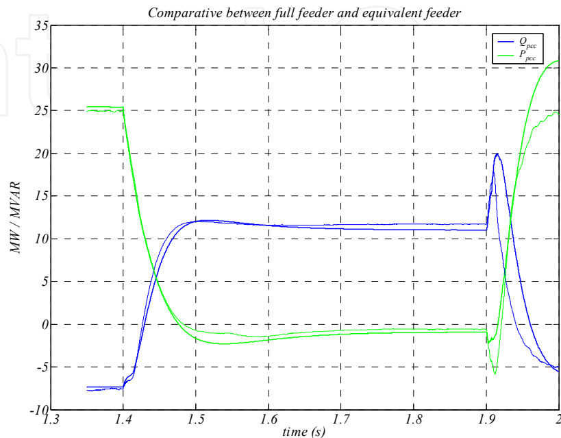
Figure F.2 Comparison of the equivalent wind turbine and the full feeder for a three-phase fault, the evolution of the active and reactive power during the fault at the PCC,
