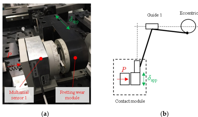
Figure 6. (a,b) The contact module for fretting wear configuration.
