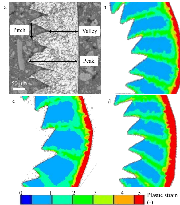
Fig. 5. Comparisons of chip morphology (all to the same scale) between a) experimental results and FEM results with b) JC, c) PL and d) Iturbe models.
