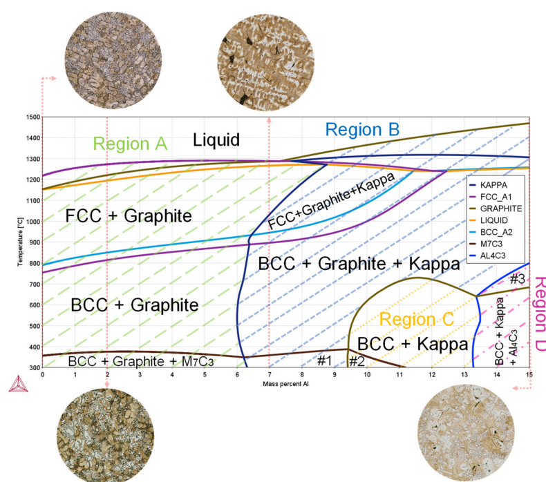
Figure 1. Phase diagram of the nominal composition of the Fe-3.1C-2.0Si-0.6Mn alloy with variable wt.% of Al correlated with the etched microstructures subsequently observed by OM (#1 = BCC + Graphite + kappa + M_7C_3 ; #2 = BCC + kappa + M_7C_3 ; #3 = BCC + kappa + M_7C_3 + Al_4C_3 ).
