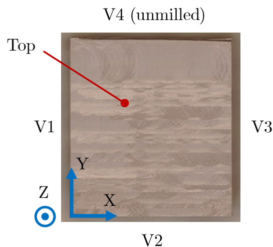
Figure 3. Names of the characterized surfaces and top view of a part; magnification 40×.
