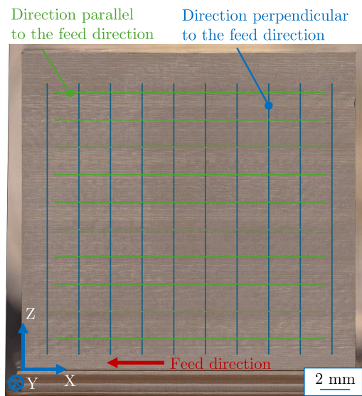
Figure 5. Directions of evaluation for the profile surface texture parameters on surface V2; magnification 40×.
