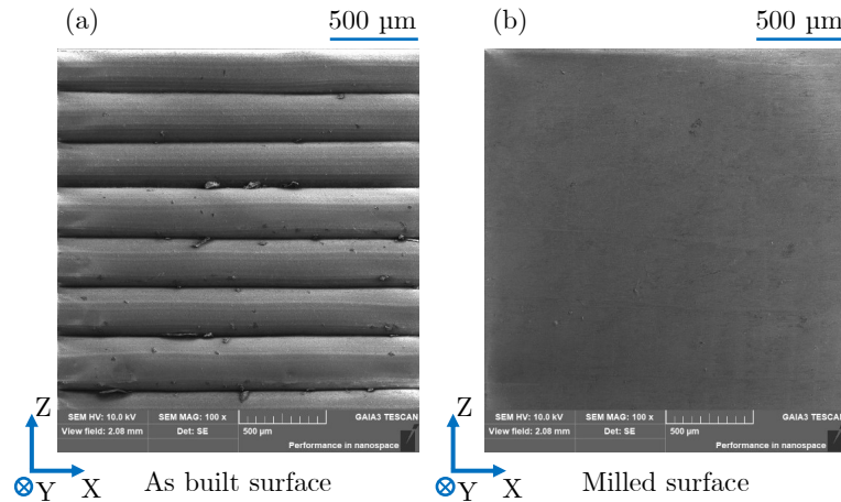
Figure 8. FIB-SEM pictures of the unmilled Vertical surface V4 after sintering (a) and the milled Vertical surface V2 after sintering (b); magnification 100×.
