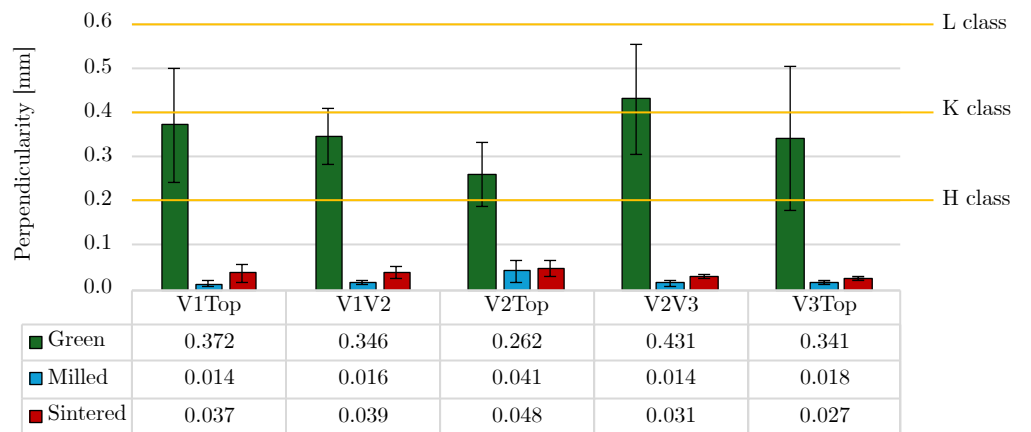
Figure 13. Perpendicularity deviation (in mm) of the part Top and Vertical surfaces for the green (after step 1), milled (after step 2) and sintered (after step 3) states of the parts.
