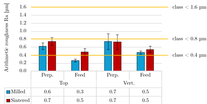
Figure 16. Arithmetic roughness (Ra in \mu\text{m} ) of the parts’ Top and Vertical surfaces for the milled (after step 2) and sintered (after step 3) states; “Perp.” stands for the direction perpendicular to the feed (“Feed”) direction.
