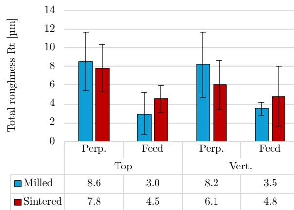
Figure 17. Total roughness (Rt in \mu\text{m} ) of the parts’ Top and Vertical surfaces for the milled (after step 2) and sintered (after step 3) states: “Perp.” stands for the direction perpendicular to the feed (“Feed”) direction.
