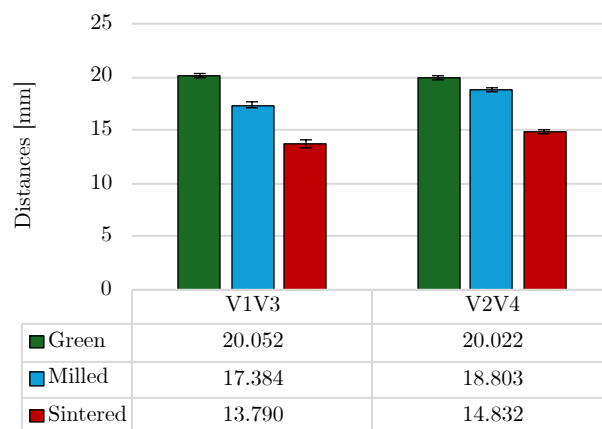
Figure 9. Vertical plane distances (in mm) for the green (as-built after step 1), milled (after step 2) and sintered (after step 3) states of the parts.
