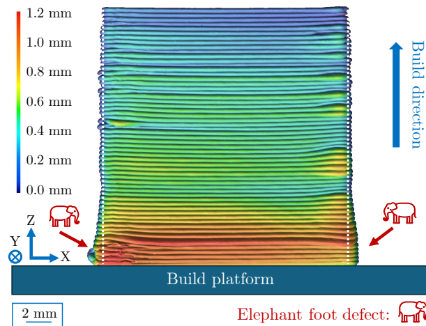
Figure 10. Elephant foot defect at the interface between the part and the build platform for surface V2; magnification 40×.
