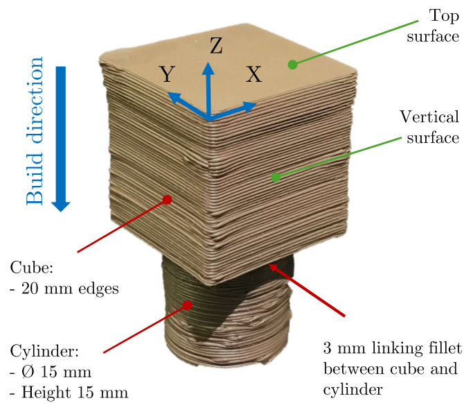
Figure 2. Selected part design.
