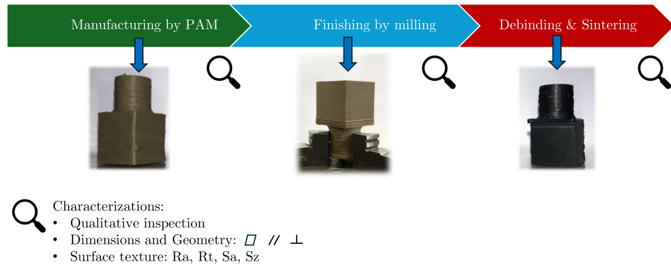
Figure 1. The three experimental steps performed as well as the manufactured part’s characteristics.
