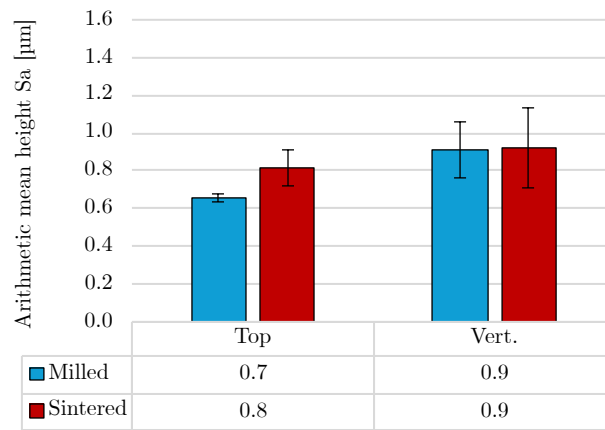
Figure 18. Arithmetic mean height (Sa in \mu\text{m} ) of the parts' Top and Vertical surfaces for the milled (after step 2) and sintered (after step 3) states.
