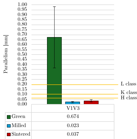
Figure 12. Parallelism deviation (in mm) between the V1 and V3 Vertical surfaces for the green (after step 1), milled (after step 2) and sintered (after step 3) states of the parts.
