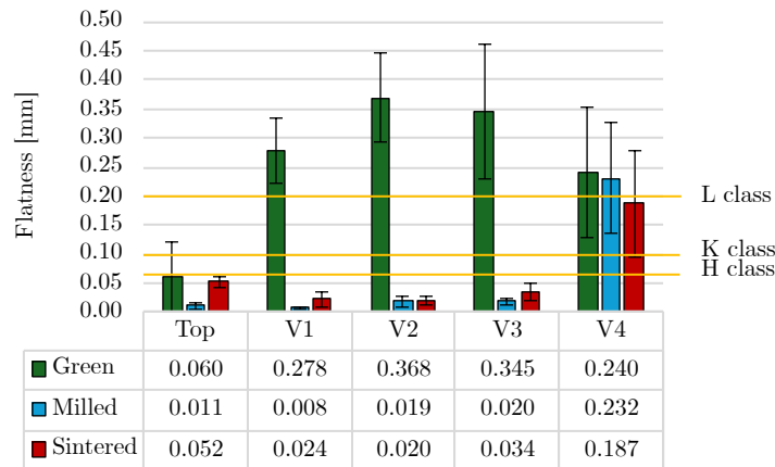
Figure 11. Flatness deviation (in mm) of the Top and Vertical surfaces (V1 to V4) for the green (after step 1), milled (after step 2) and sintered (after step 3) states of the parts.
