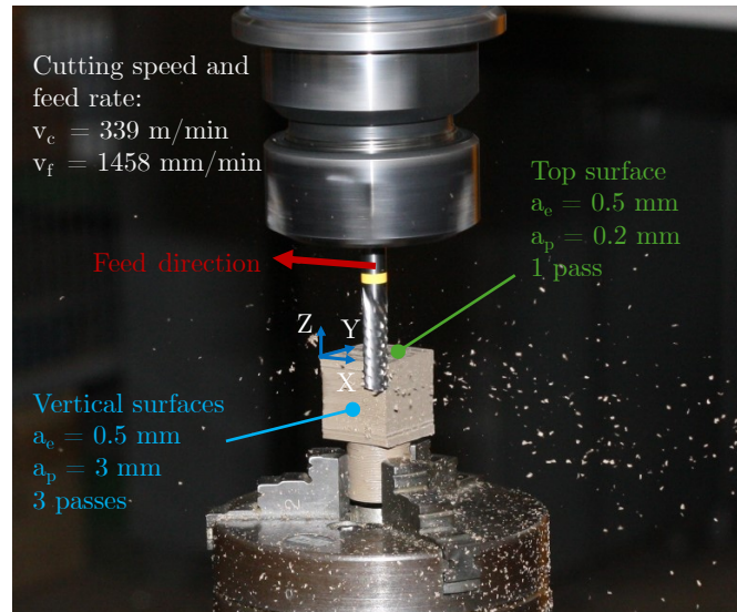
Figure 4. The parameters and configuration of the milling operation—finishing of a Vertical surface.
