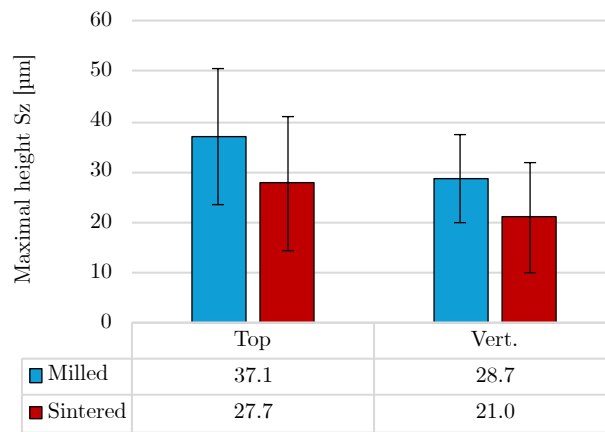
Figure 19. Maximum height (Sz in \mu\text{m} ) of the parts' Top and Vertical surfaces for the milled (after step 2) and sintered (after step 3) states.
