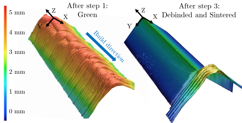
Figure 7. Qualitative view of a part's corner at the green state (after step 1) and after the debinding and sintering operations (after step 3); magnification 40×.
