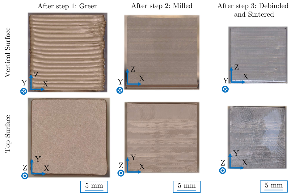
Figure 6. Qualitative evaluation of the parts' Vertical (V2) and Top surfaces at the green (as-built after step 1), milled (after step 2) and sintered (after step 3) states; magnification 40×.
