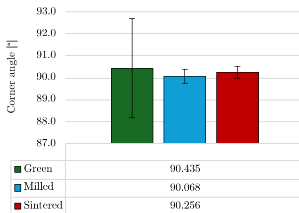
Figure 14. Corner angle (in degrees) between the Vertical surfaces of the parts for the green (after step 1), milled (after step 2) and sintered (after step 3) states.
