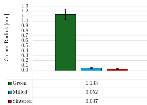
Figure 15. Corner radii (in mm) between the Vertical surfaces of the parts for the green (after step 1), milled (after step 2) and sintered (after step 3) states.
