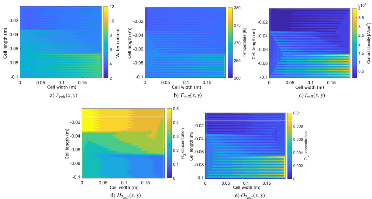
Fig. 10 – Spatial distribution of the most relevant variables at the high-performance operation point.
