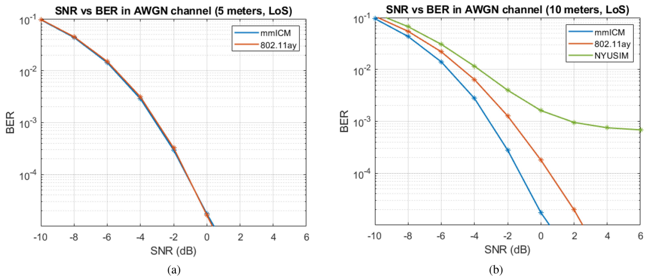
FIGURE 12. Performance of an 802.11ad link evaluated with the mmICM, 802.11ay and NYUSIM models. (a) Performance at 5 meters. (b) Performance at 10 meters.
