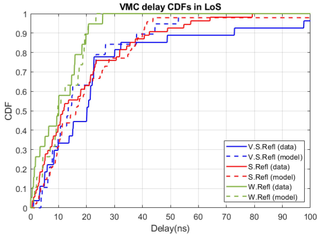
FIGURE 10. Reflector excess delay CDF in VMC LoS.
