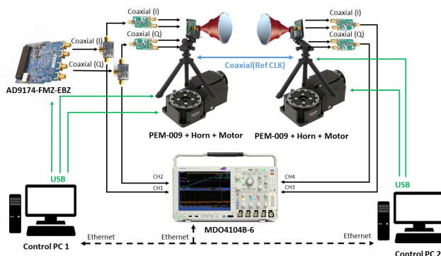
FIGURE 1. General picture of sounding system.
