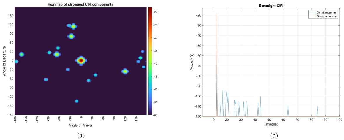
FIGURE 9. Example CIR generated with the model. (a) Heatmap of maximum gain per direction. (b) Bore-sight CIR of directional/omni antennas.
