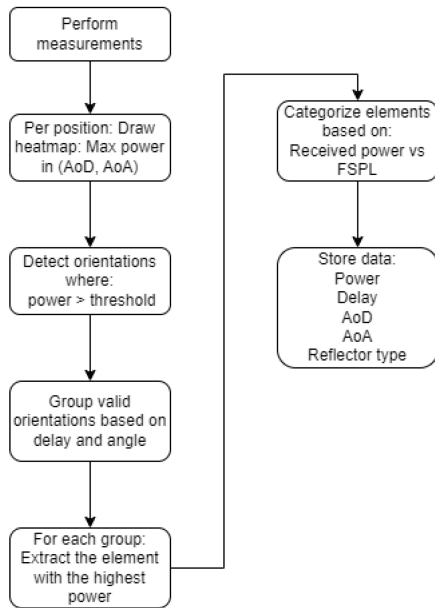
FIGURE 6. Flowchart of postprocessing steps.
