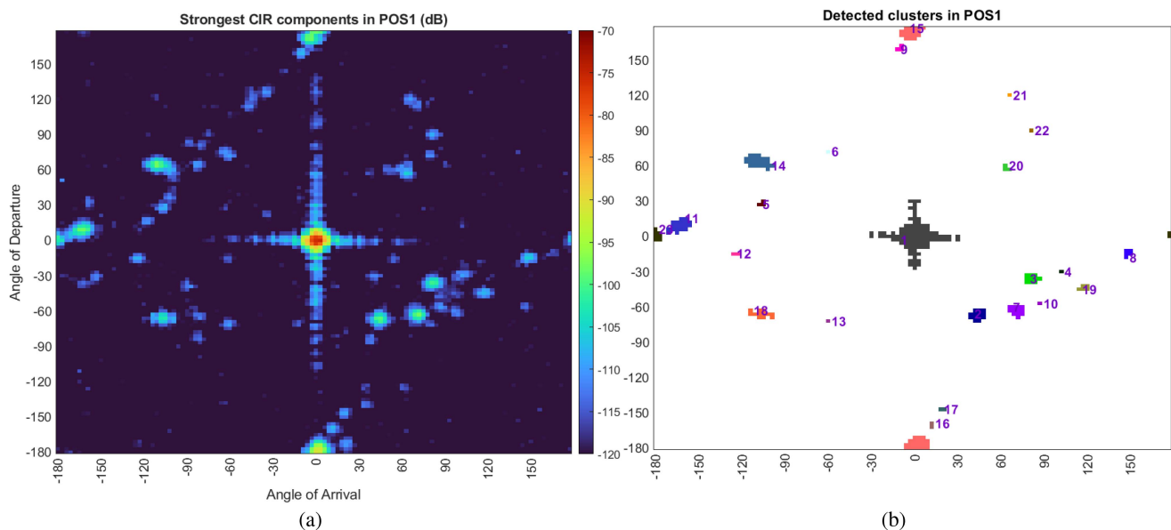
FIGURE 7. Maximum power heatmap and detected reflectors in position 1. (a) Maximum power heatmap. (b) Detected reflectors.
