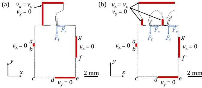
Figure 4. Mechanical boundary conditions and 1/3 rd scale workpiece, for (a) single and (b) two-tooth tool simulations. Lengths ab, de, fg to scale.
