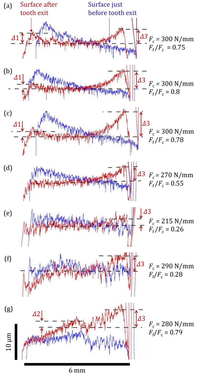
Figure 5. Surface profiles and their accompanying F_c, F_t/F_c values, (a-f) single and (g) two-tooth simulations. Input conditions: (a) \gamma = -5^\circ, \mu = 0.9, E_{work} = E_{tool} = 220 GPa, (b-f) as in (a) but with conditions changed as follows: (b) E_{tool} = 2200 GPa, (c) E_{tool} = 2200 GPa, and E_{work} = 150 GPa, (d) \gamma = 10^\circ , (e) \gamma = 30^\circ , (f) as in (e) but flow stress increased 50%, and (g) as in (a). The colour scheme and scale are the same for all parts.
