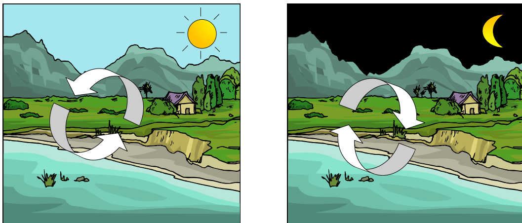
Figure 2-2: Illustration of the sea breezes direction.
