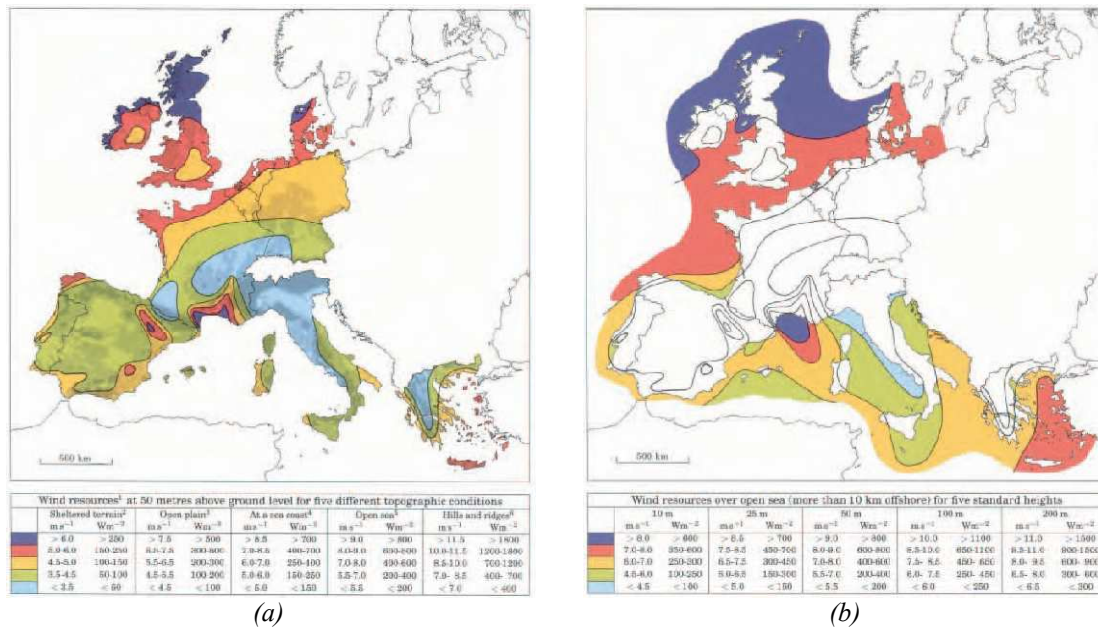
Figure 2-17: The average wind speed in Europe, in land (a) and offshore (b) [ 20 ].
