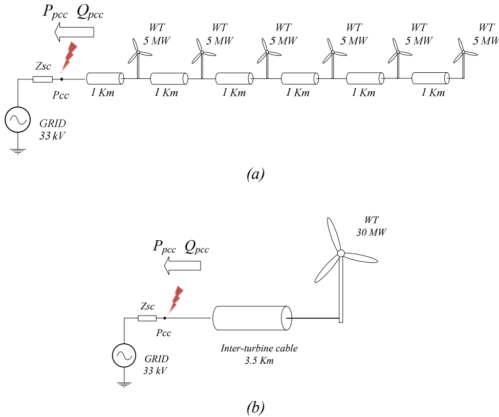
Figure F-1: Considered simulation scenarios to validate the simplification. (a) Full feeder and (b) equivalent wind turbine.
