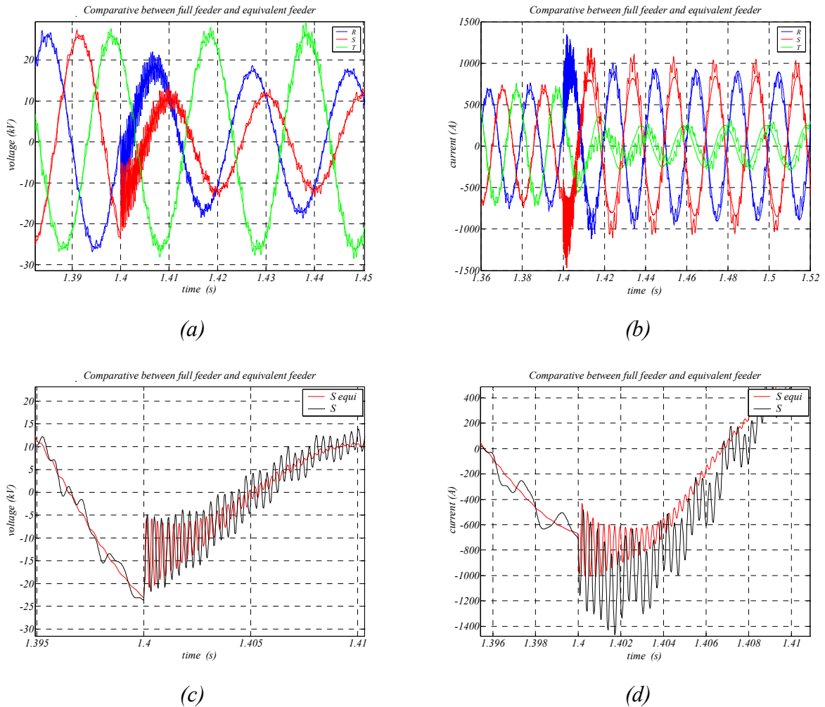
Figure F-9: Comparison of the equivalent wind turbine and the full feeder for a two-phase fault. the voltage (a) and current (b) at the PCC the same instant that the fault occurs, (c)-(d) at the same instant of the fault mono-phase and more detailed (red, equivalent feeder).
