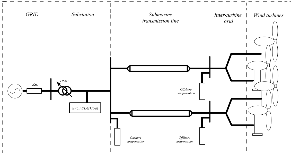
Figure 3-3: Typical layout of multiple MVAC transmission system.
