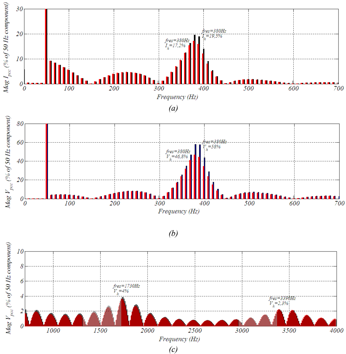
Figure 6-23: Frequency response of the equivalent wind farms model via PSCAD. Frequency response from the viewpoint of the equivalent wind turbine closest the collector point (red) and for the equivalent wind turbine 5.5 Km away the collector point (Blue). FFT of the current (a) and FFT of the voltage (b)-(c).
