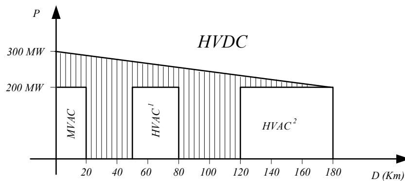
Figure 3-6: Optimum configuration depending on distance to shore and rated power: (1) With reactive compensation at both ends, (2) With reactive compensation at both ends and another one in the middle of the submarine cable.
