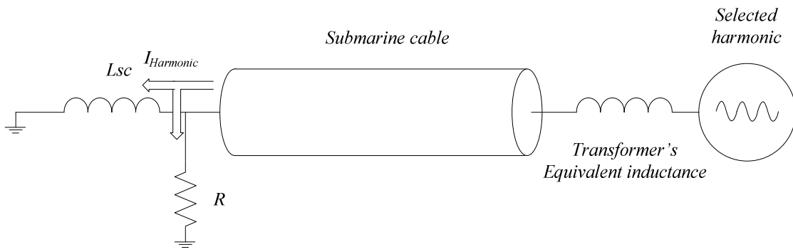
Figure E-2: Transmission system with an RLC filter at the resonance frequency of the filter.
