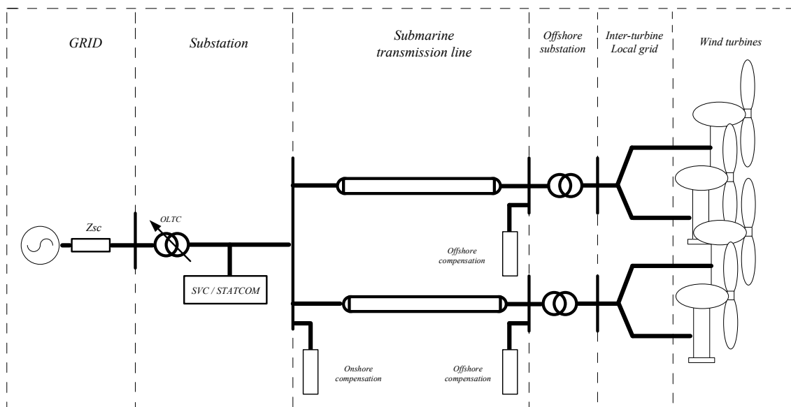
Figure 3-4: Typical layout of multiple HVAC transmission system.
