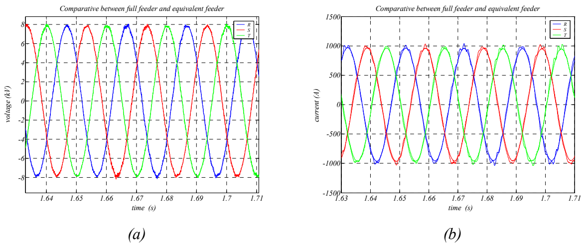
Figure F-5: Comparison of the equivalent wind turbine and the full feeder for a three-phase fault, the voltage (a) and current (b) at the PCC during the maintenance of the fault.
