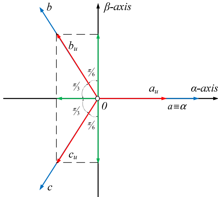
Figure D-1: Vector representation of the abc to \alpha\beta transform.
