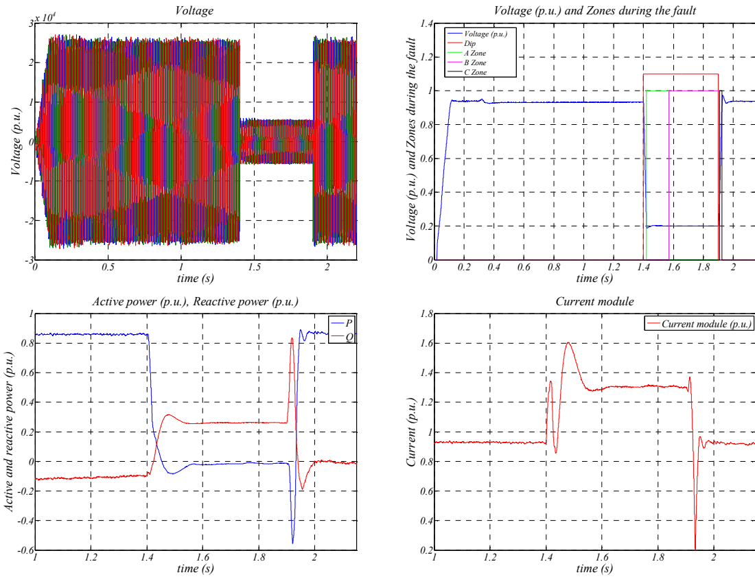
Figure 5-19: Summarized graphical results of a 2 nd category fault for the test defined in the PVVC, voltage (module and signals), power and current results.
