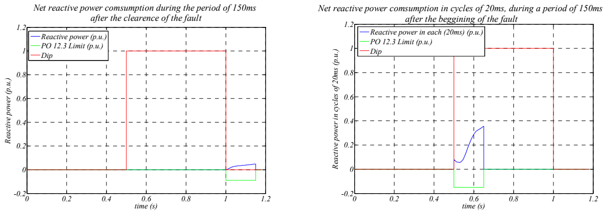
Figure 7-37: Summarized graphical results of a 2 nd category fault for the test defined in the PVVC, reactive power consumption in C zone and A zone.
