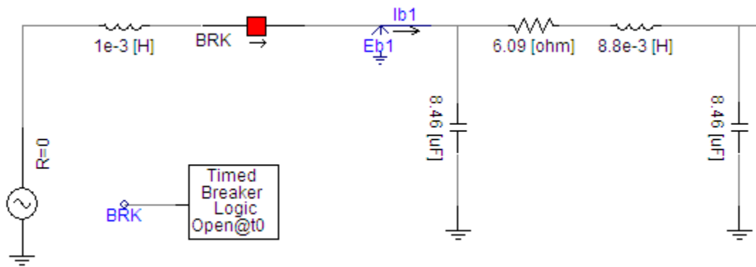
Figure 4-27: Simulation scenario in PSCAD for the “π” circuit.
