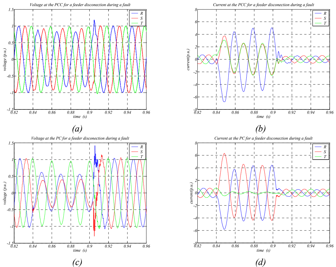
Figure 7-14: Three-phase signals (current and voltage) at the main points of the considered wind farm when a feeder is disconnected during a short circuit fault.
