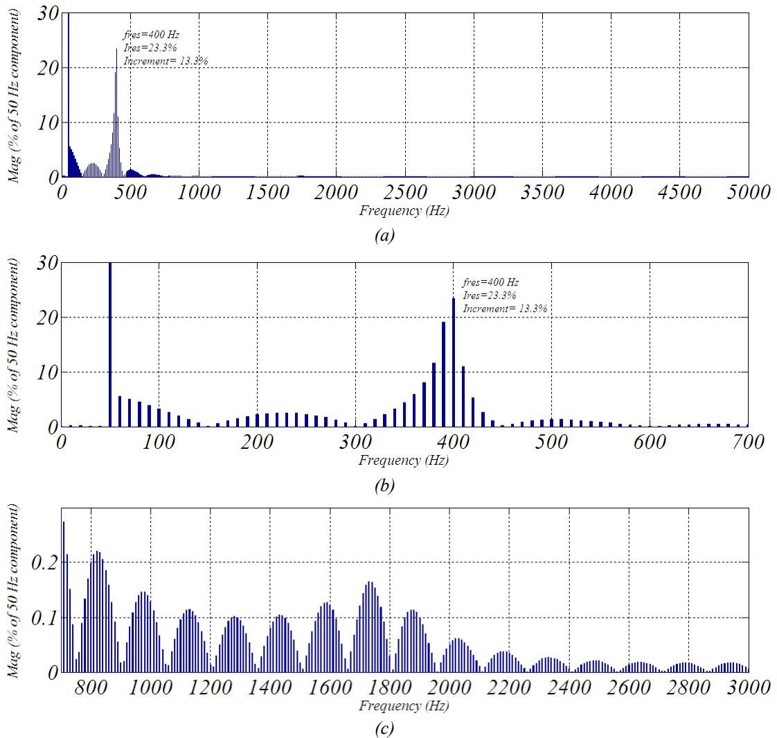
Figure 6-5: Frequency response of the transmission system with only: step-up transformer and submarine cables. FFT of the current at PCC. (a) Whole analyzed spectrum, (b) more detail in the main resonance and (c) more detail in high frequencies.
