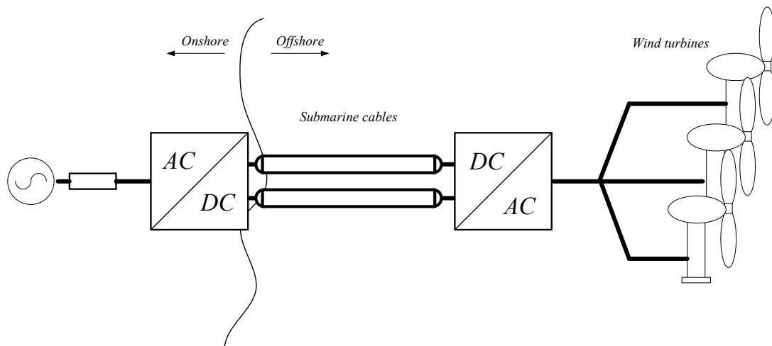
Figure 3-5: Generic layout of bipolar HVDC transmission system.
