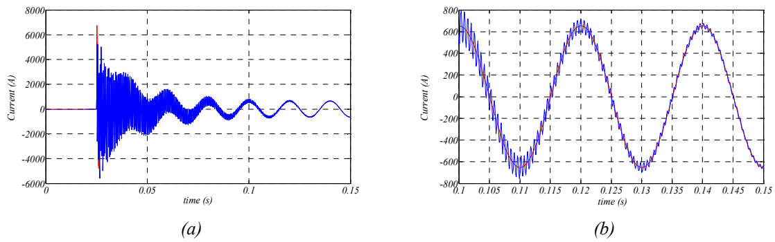
Figure 4-29: Comparison of the input current of the cable (Ib1): (blue) for the "π" circuit and (red) for the frequency-dependent model in phase domain of PSCAD.
