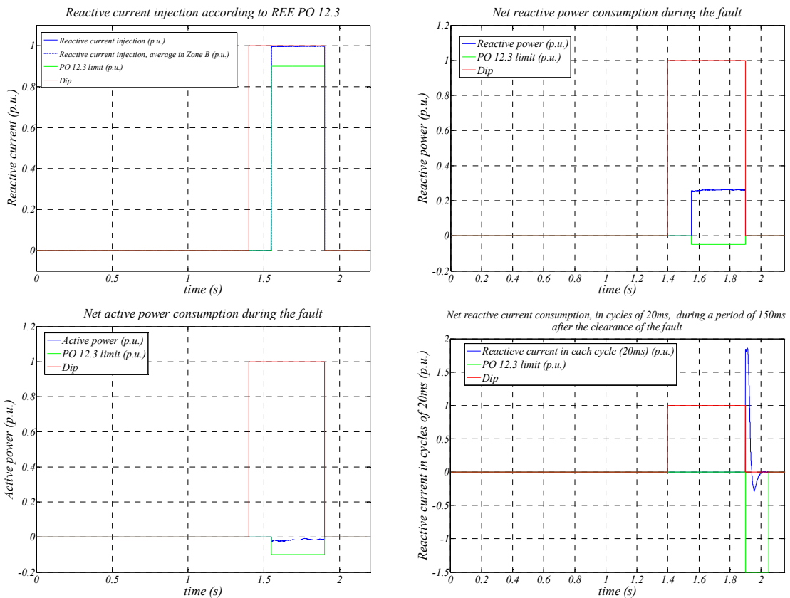
Figure 5-20: Summarized graphical results of a 2 nd category fault for the test defined in the PVVC, reactive current and power consumption in B zone and reactive current consumption in C zone.
