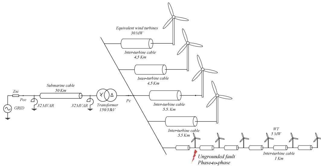
Figure 7-13: The scheme of the simulation scenario used to evaluate the effect of the disconnection of a feeder during a short circuit fault (phase to phase).
