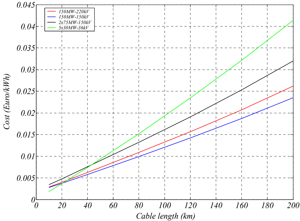
Figure 5-8: Energy transmission cost for different layouts.
