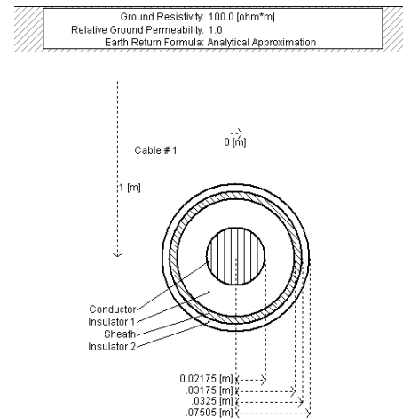
Figure 4-26: Graphic representation of the cable in PSCAD and its parameters.
