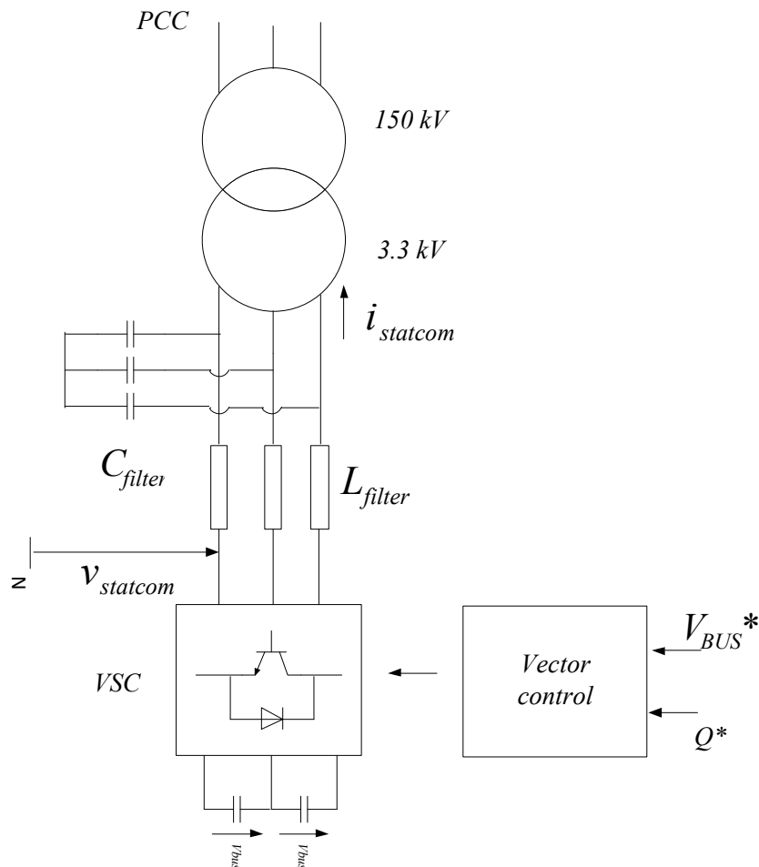
Figure G-1: Main scheme of the considered STATCOM used to validate the proposed electric connection infrastructure.
