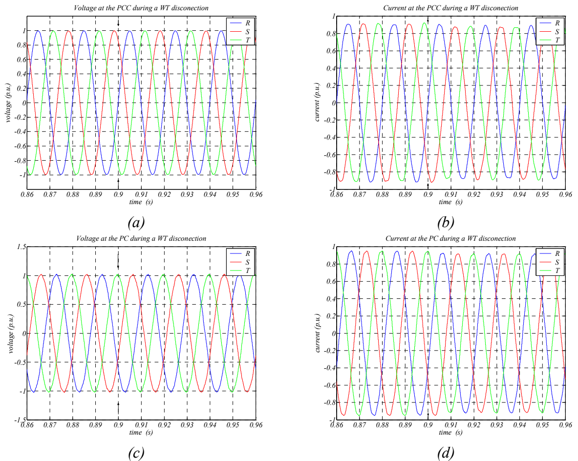
Figure 7-10: Three-phase signals (current and voltage) at the main points of the considered wind farm when the disconnection of a wind turbine occurs.
