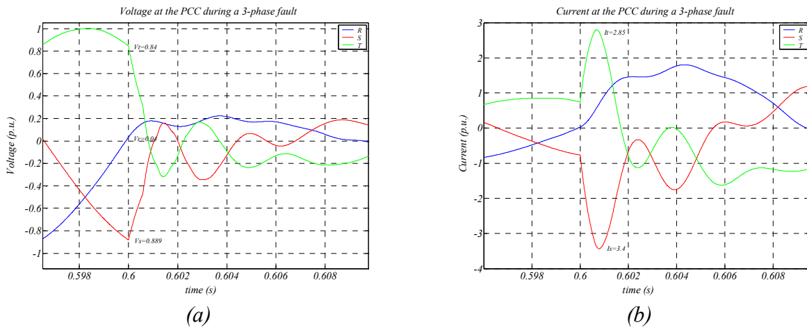
Figure 7-23: Current and voltage in detail at the PCC when the fault happens (0.6s).
