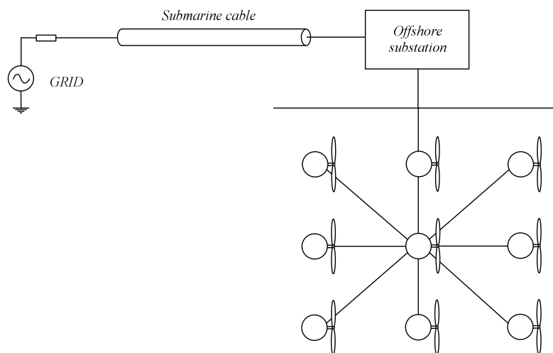
Figure 3-10: Layout of the star design for local inter-turbine grid.
