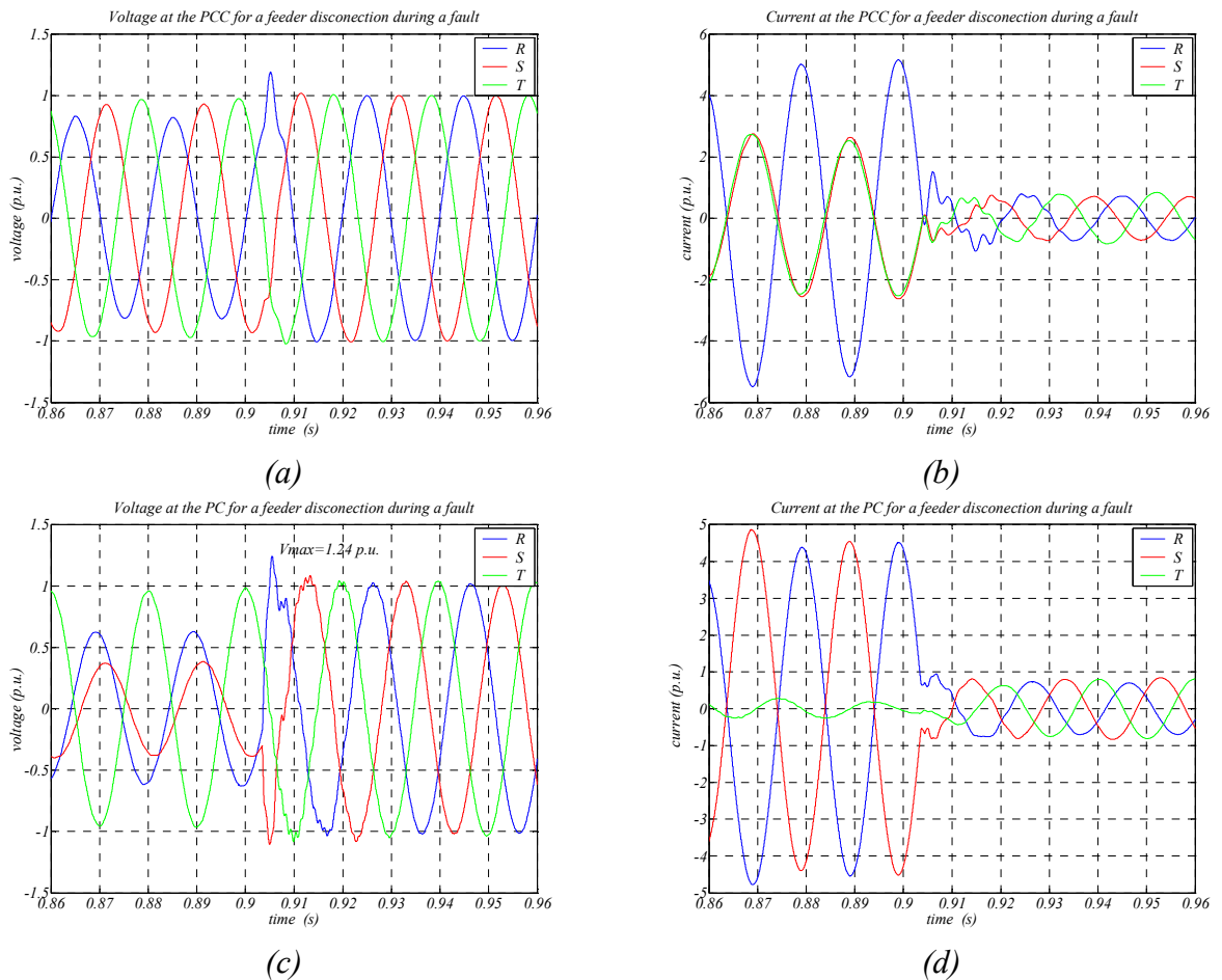
Figure 7-19: Three-phase signals (current and voltage) at the main points of the considered wind farm with passive filters when the disconnection of a feeder occurs during a fault.
