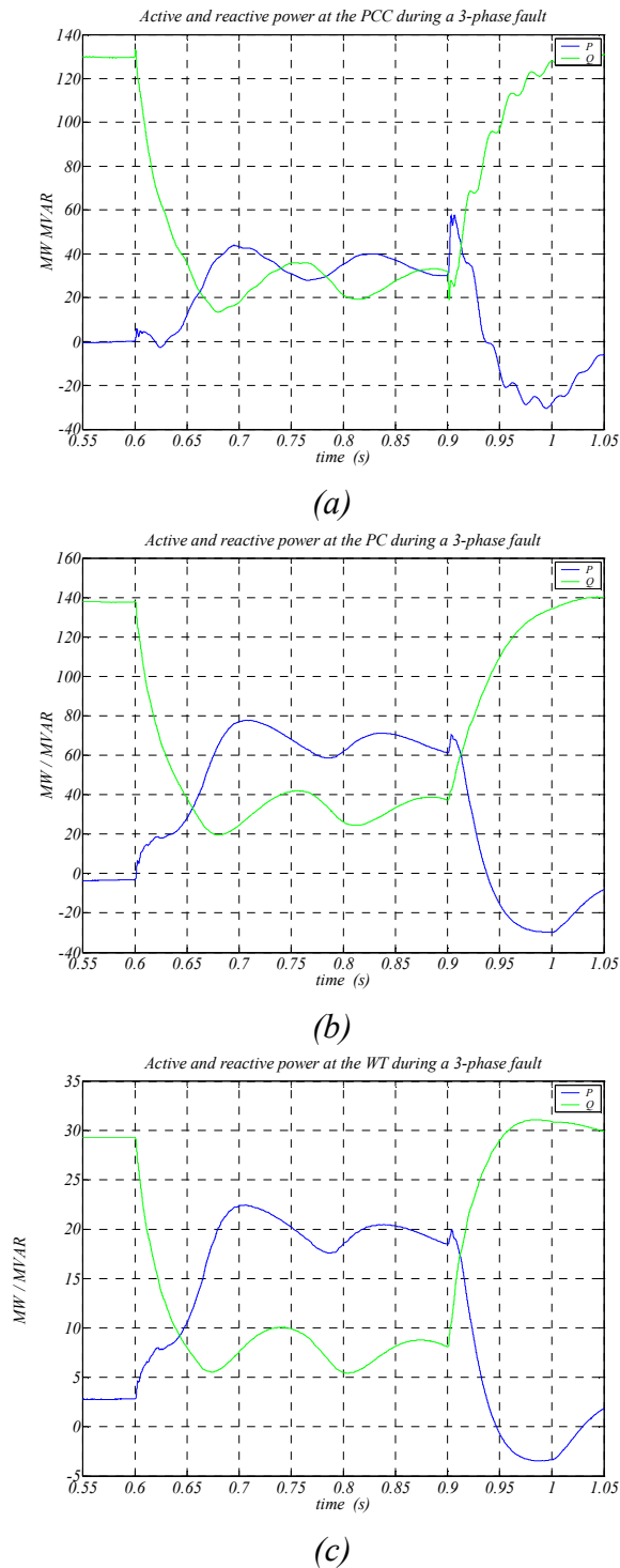
Figure 7-26: Active and reactive power at the main points of the simulation scenario, (a) PCC, (b) PC and (c) at the terminals of the wind turbine.
