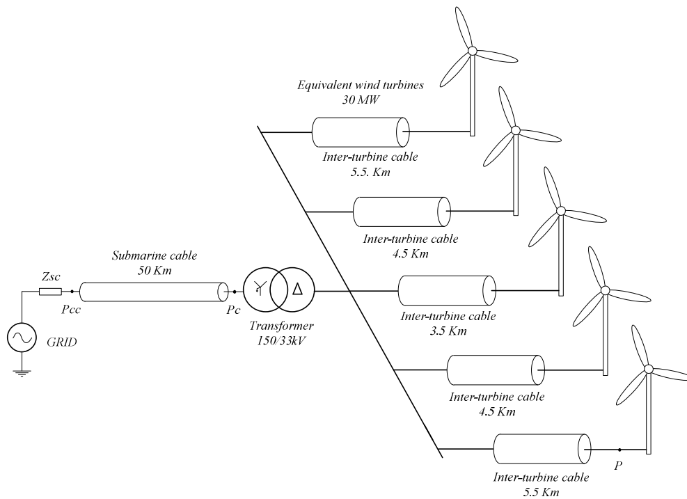
Figure 6-22: Diagram of the simulation scenario with wind turbine models.
