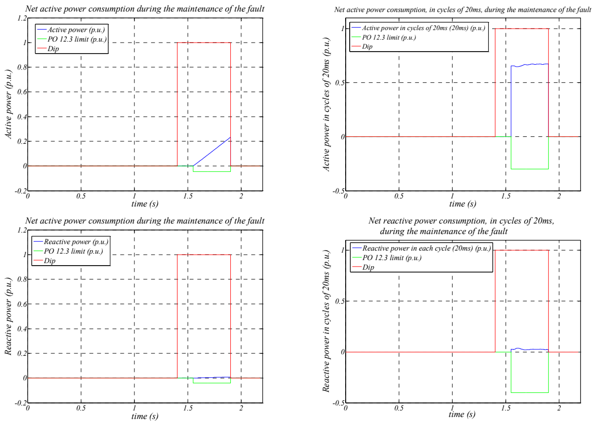
Figure 5-23: Summarized graphical results of a 4 th category fault for the test defined in the PVVC, active and reactive power consumption in B zone.
