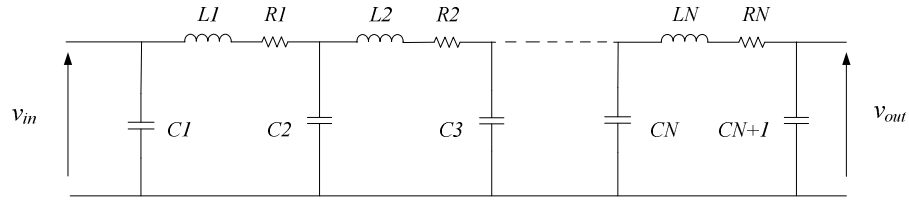
Figure 4-20: Submarine cable modeled as N “π” circuits.
