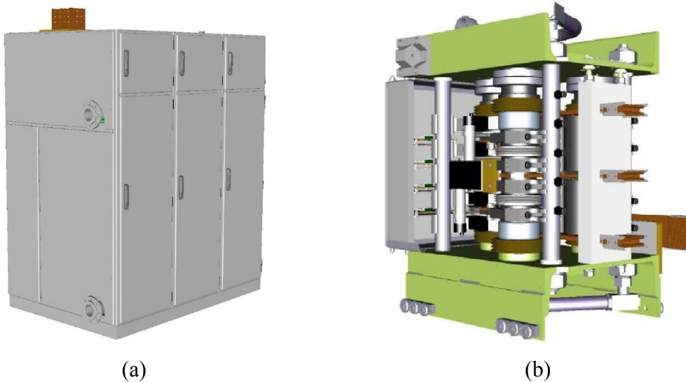
Figure 5-11: (a) External appearance of the Ingedrive MV 300 of Ingeteam and (b) The basic power module (BPM) equivalent to a branch of the three-level converter, the module is composed by 4 IGBTs, 4 weeling diodes and 2 clamp diodes, all of them based on IEGTs technology.
