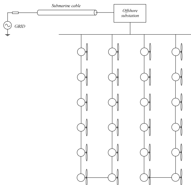
Figure 3-9: Layout of the double sided ring design for local inter-turbine grid.
