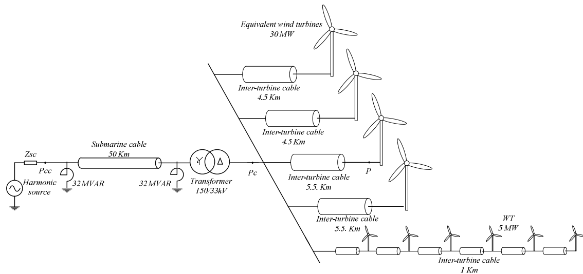
Figure 7-7: Considered scenario for the problem assessment.
