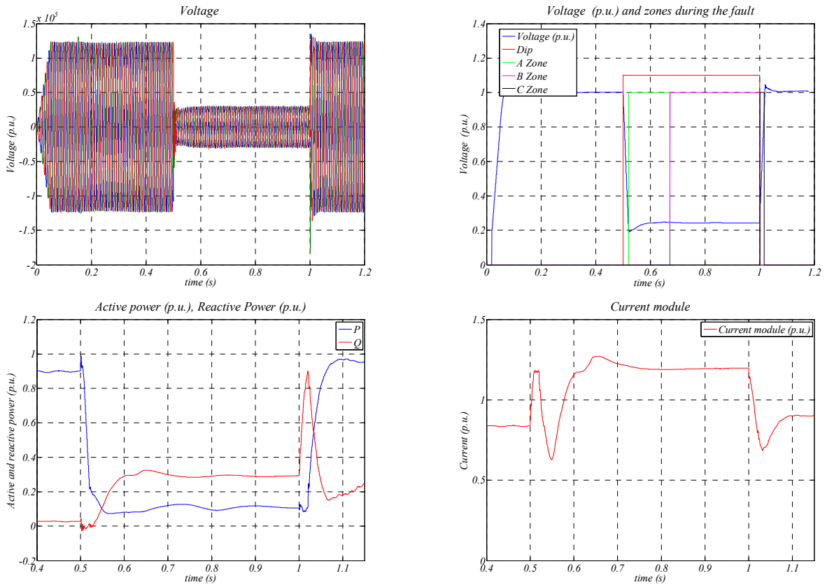
Figure 7-35: Summarized graphical results of a 2 nd category fault for the test defined in the PVVC, voltage (module and signals), power and current results..
