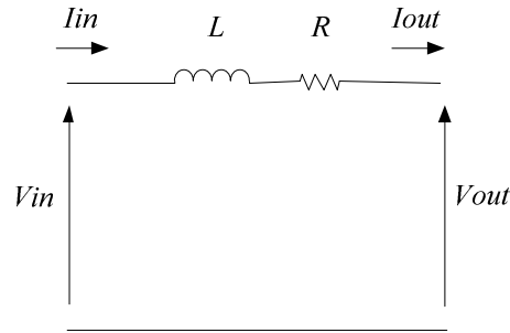
Figure 4-17: Standard cable model for short lengths.
