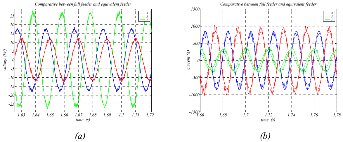
Figure F-10: Comparison of the equivalent wind turbine and the full feeder for a two-phase fault, the voltage (a) and current (b) at the PCC during the maintenance of the fault.
