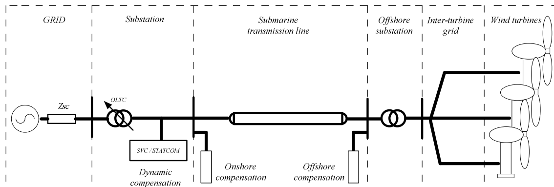
Figure 3-2: Typical layout of HVAC transmission system.
