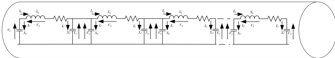
Submarine cable
