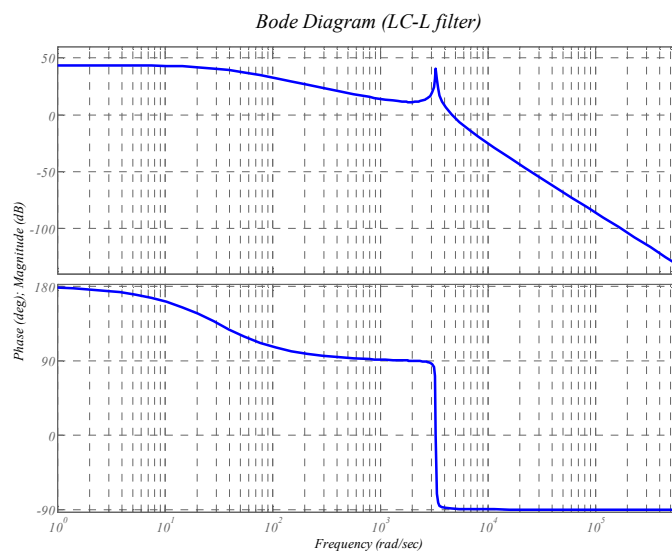
Figure 5-15: Bode diagram of the LC-L filter.
