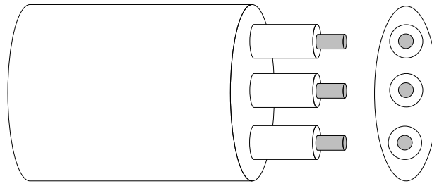
Figure 4-5: Conductor with multiple conductive elements.
