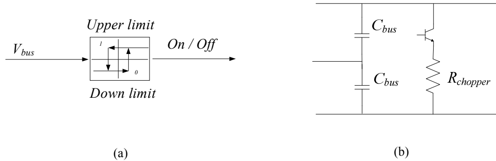
Figure 5-12: (a) Control block diagram (On/Off) of the DC chopper. (b) Electric lay-out of the considered chopper circuit.
