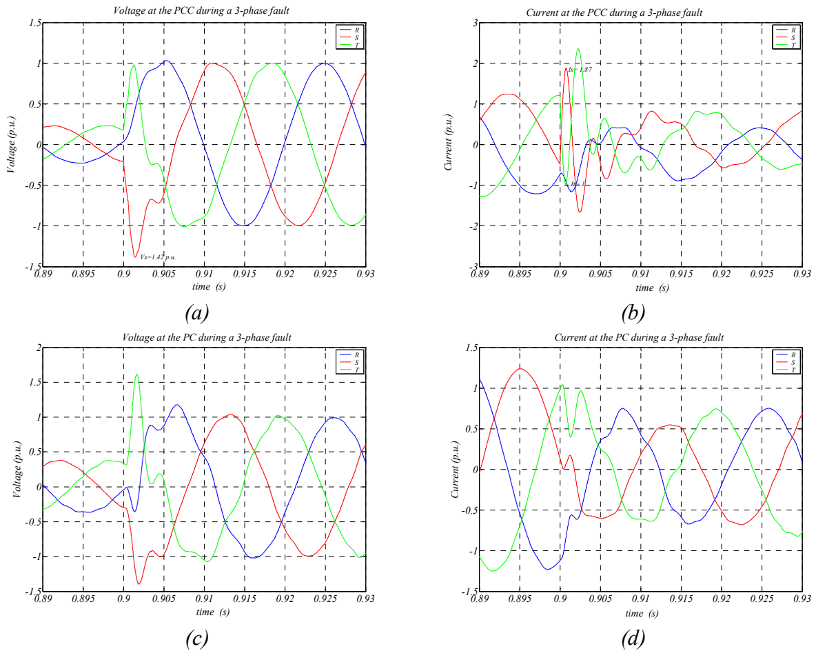
Figure 7-24: Current and voltage in detail at the PCC (a) – (b) and PC (c) – (d), when the fault is cleared (0.9s).
