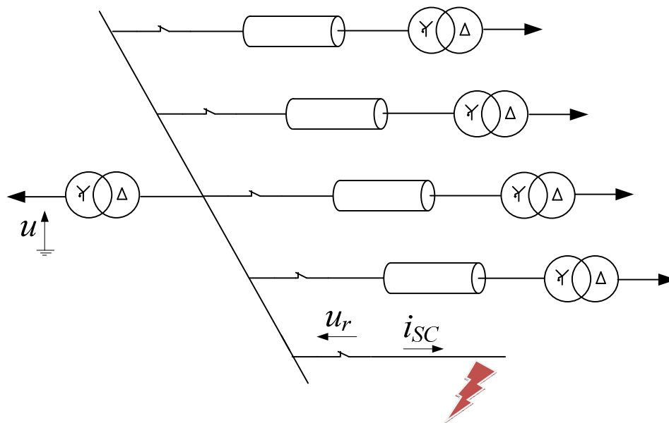
Figure 7-1: Generic large substation composed by several feeders.
