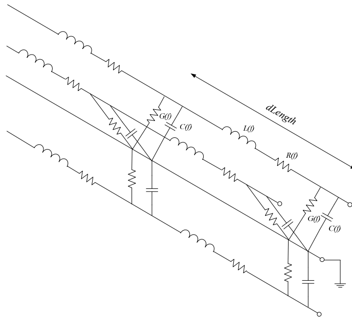
Figure 4-13: Electrical representation of a three-phase cable per differential length with frequency dependent parameters.
