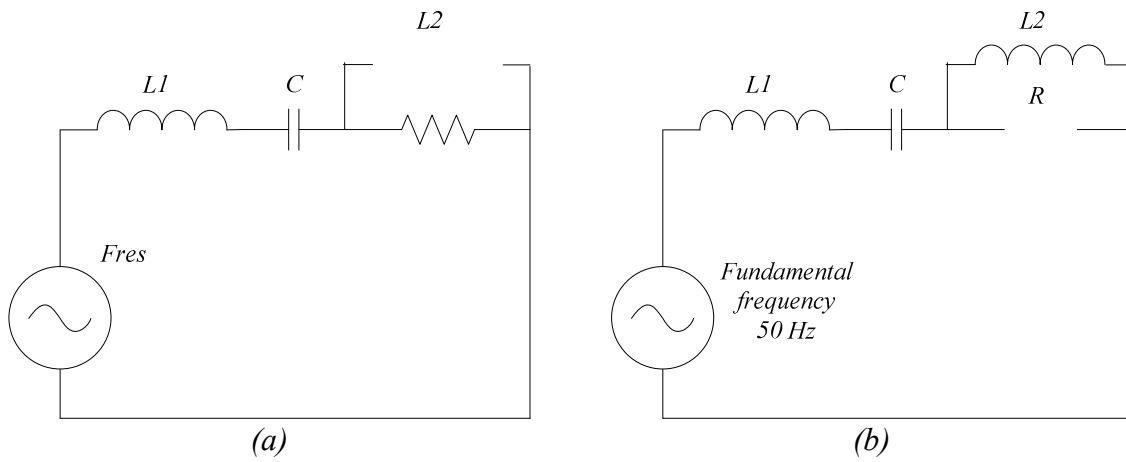
Figure E-8: Equivalent (R+L)LC circuit approximation depending on the frequency, (a) At resonance frequency and (b) at fundamental frequency.
