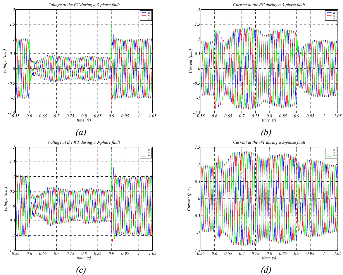
Figure 7-25: Current and voltage at the PC (a) – (b) and wind turbine terminals (c) – (d), three-phase signals.
