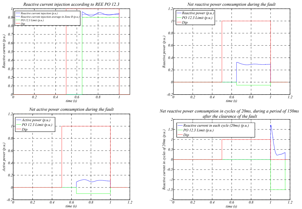
Figure 7-36: Summarized graphical results of a 2 nd category fault for the test defined in the PVVC, reactive current and power consumption in B zone and reactive current consumption in C zone.
