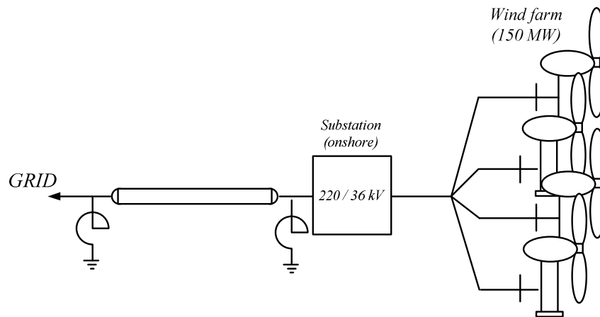
Figure 5-1: Electric configuration of a 150MW-220kV wind farm.
