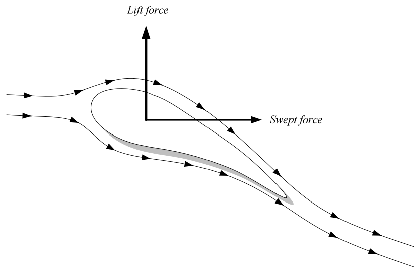
Figure 2-7: Representation of lift force and swept force generated on the blades.
