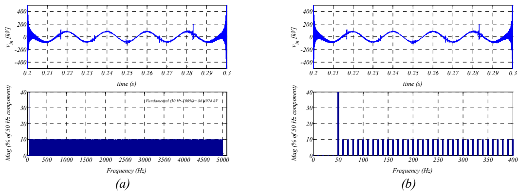
Figure 6-2: Harmonic voltage train applied to the submarine cable model. Resolution 10 Hz.
