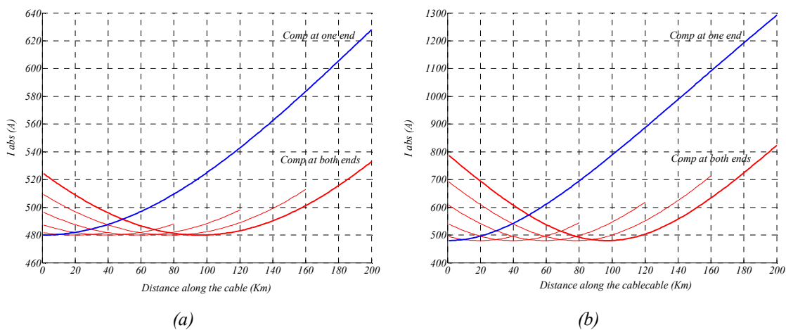
Figure 4-39: Total current along the submarine cable depending on cable length, compensation at both ends (red) and onshore compensation only (blue). (a) 30MW-36kV configuration and (b) 150MW-150kV.
