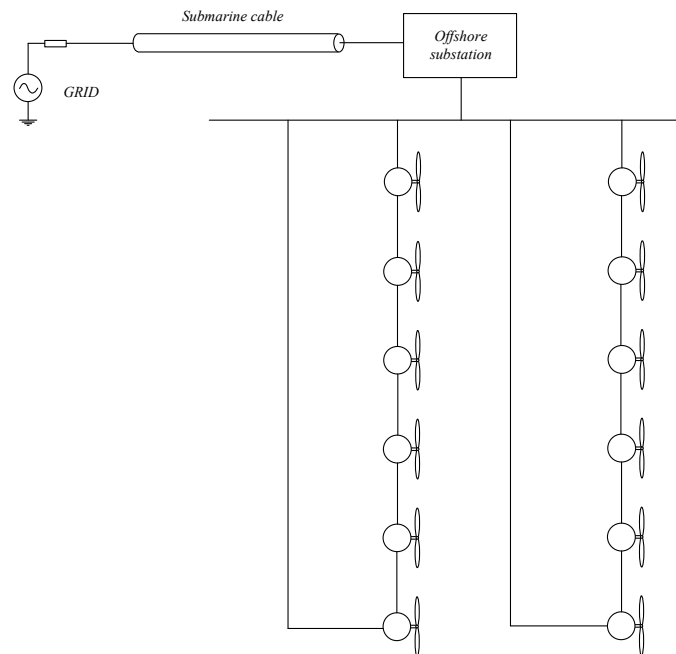
Figure 3-8: Layout of the single sided ring design for local inter-turbine grid.
