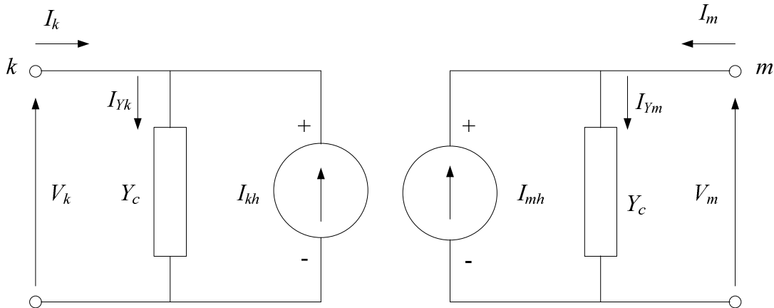
Figure 4-24: Equivalent circuit for the idempotent model.
