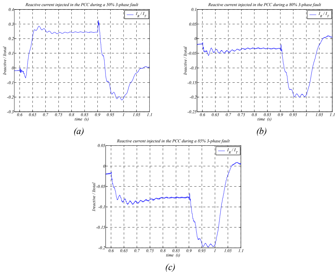
Figure 7-29: Ireactive / Itotal ratio at the PCC, (a) during a 3-phase 50% voltage dip, (b) during a 3-phase 20% voltage dip and (c) during a 3-phase 15% voltage dip.
