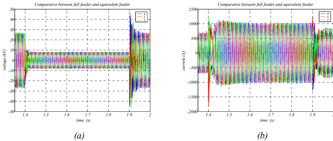
Figure F-3: Comparison of the equivalent wind turbine and the full feeder for a three-phase fault, the evolution of the voltage (a) and current (b) during the fault and the clearance at the PCC.
