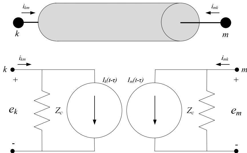
Figure 4-22: Equivalent model for Bergeron’s travelling wave.
