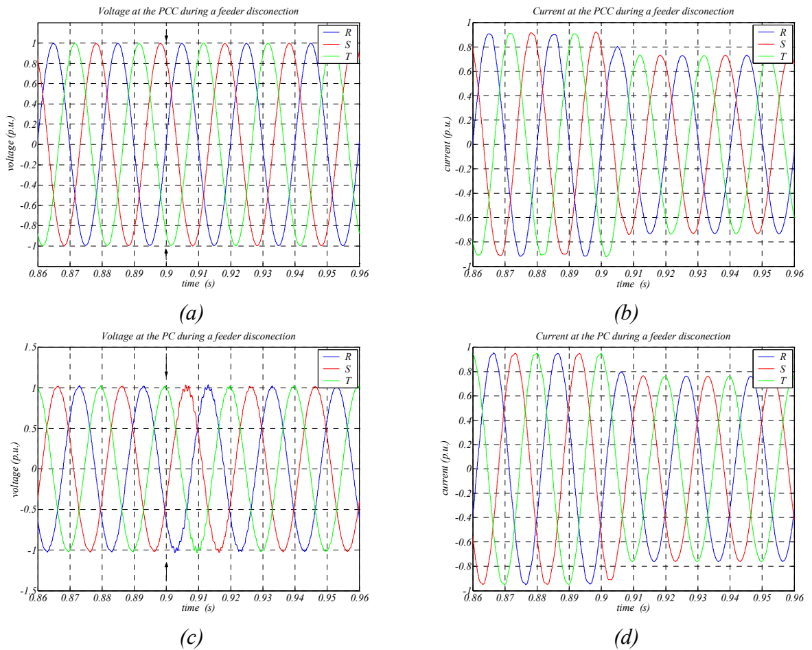
Figure 7-12: Three-phase signals (current and voltage) at the main points of the considered wind farm when the disconnection of a feeder occurs.
