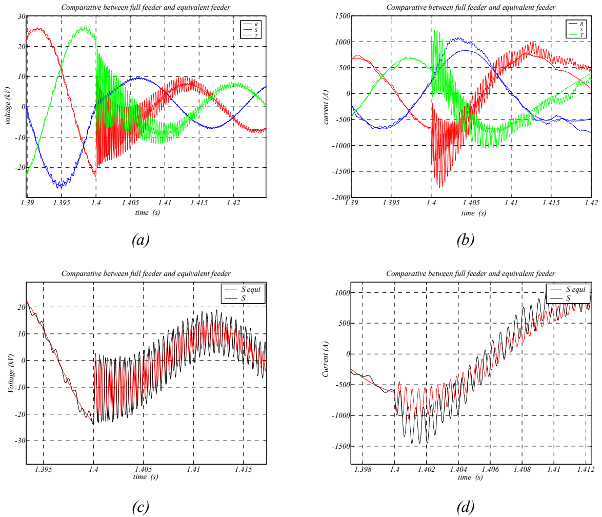
Figure F-4: Comparison of the equivalent wind turbine and the full feeder for a three-phase fault, the voltage (a) and current (b) at the PCC the same instant that the fault occurs, (c)-(d) at the same instant of the fault mono-phase and more detailed (red, equivalent feeder).
