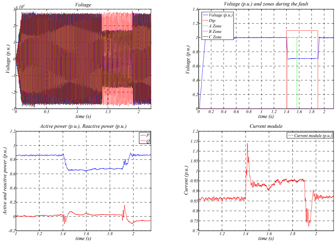
Figure 5-22: Summarized graphical results of a 4 th category fault for the test defined in the PVVC, voltage (module and signals), power and current results.
