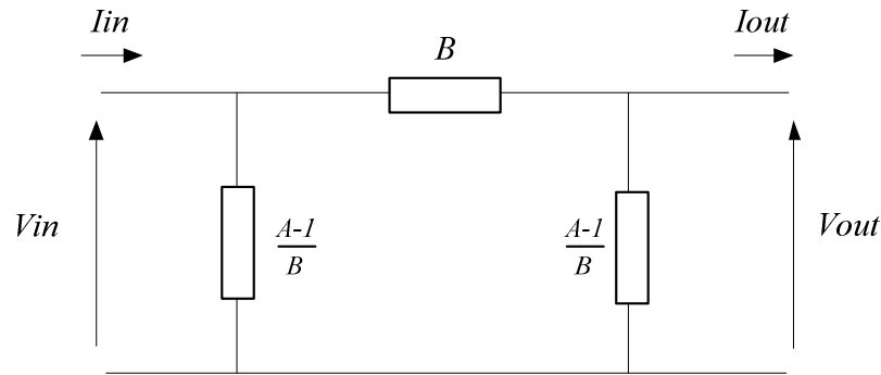
Figure 4-19: Standard cable model for long cable lengths. Equivalent \pi circuit.
