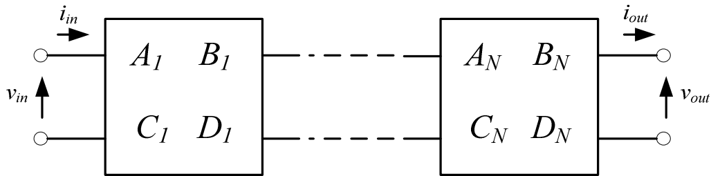
Figure 4-21: N quadrupoles in series.
