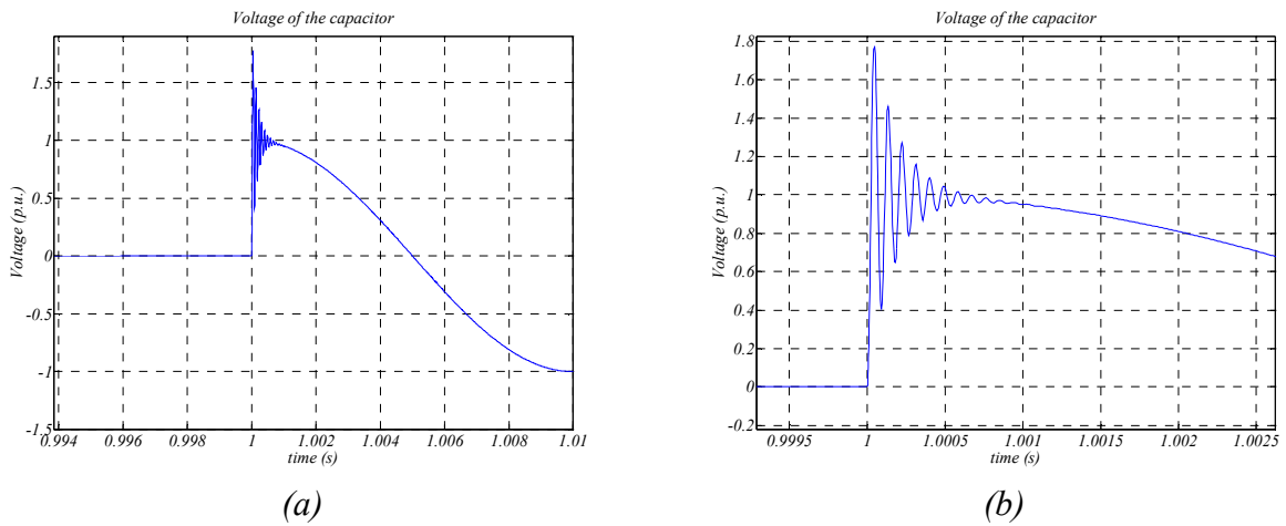
Figure 7-4: Transient voltage of the capacitor during the energizing the RLC circuit, (a) Voltage on the capacitor and (b) voltage on the capacitor with more detail around the energizing.
