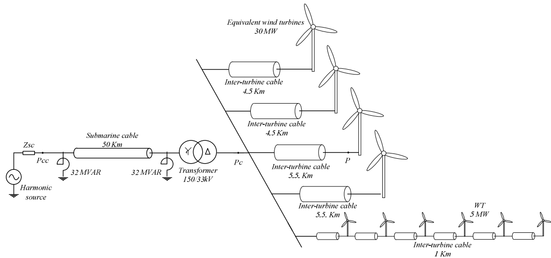
Figure 7-15: The scheme to estimate the frequency response of the considered scenario to evaluate disconnections of wind turbines and feeders.
