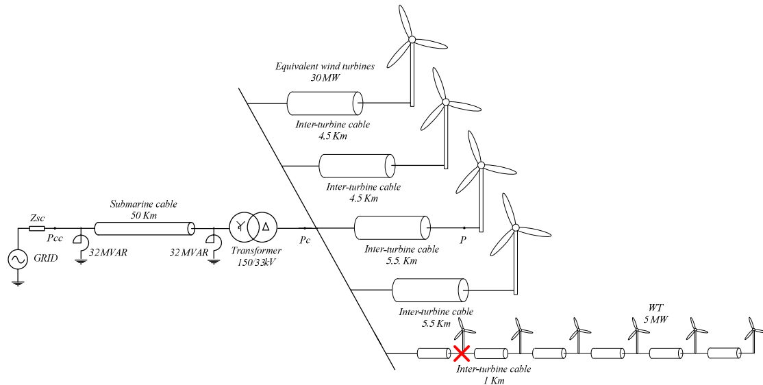
Figure 7-9: The scheme of the simulation scenario to evaluate the effect of the disconnection of a wind turbine.
