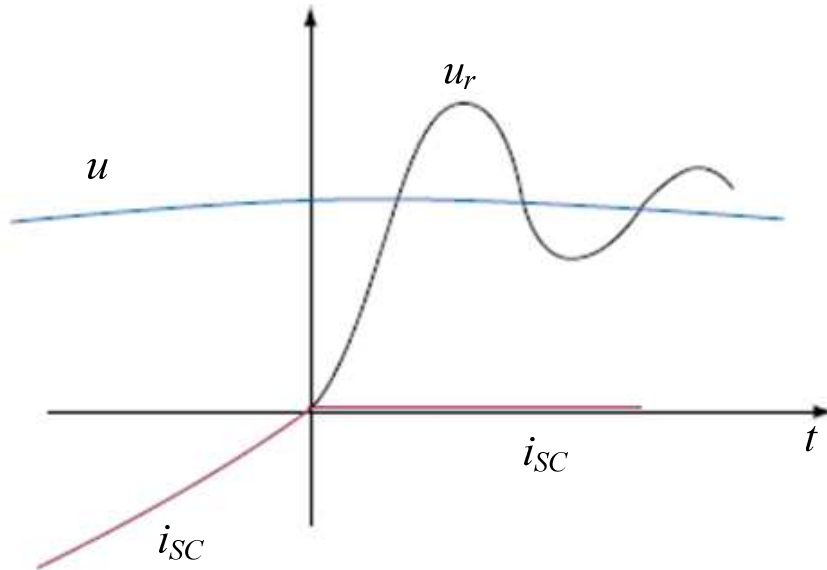
Figure 7-2: TRV for the considered network.
