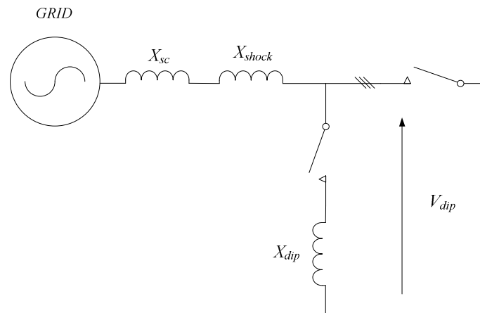
Figure 5-17: Defined test scheme in the PVVC to measure the depth of the voltage fault.
