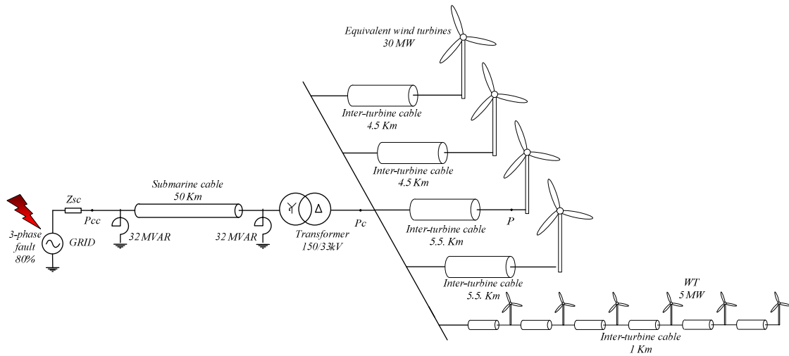
Figure 7-21: The simulation scenario to evaluate the behavior of the wind farm upon voltage dips.
