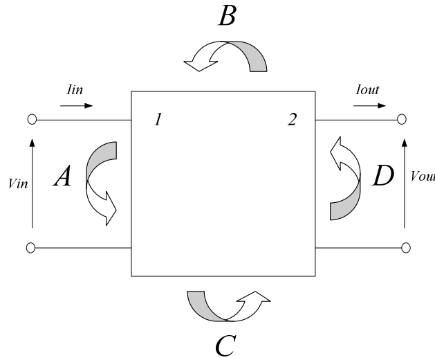
Figure 4-16: Two port system or quadripole oriented to a transmission line in phasor domain.
