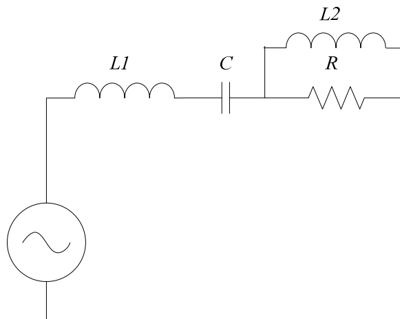
Figure E-7: Generic (R+L)LC circuit.
