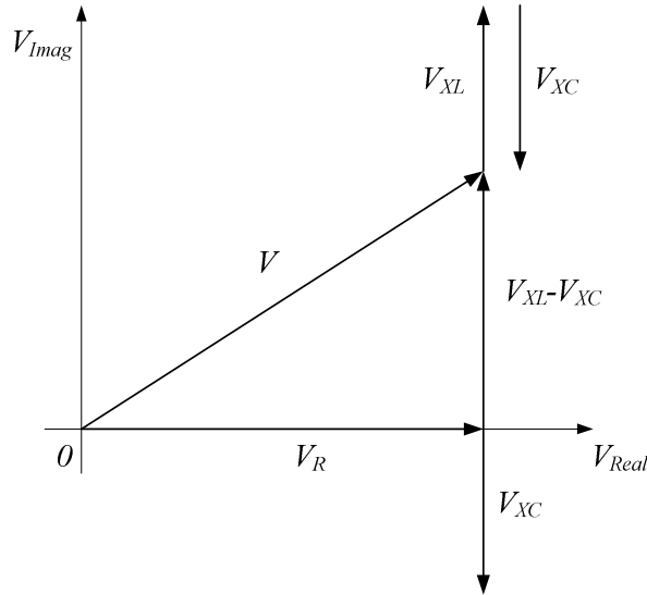
Figure E-4: Diagram of the voltages of the RLC branch.
