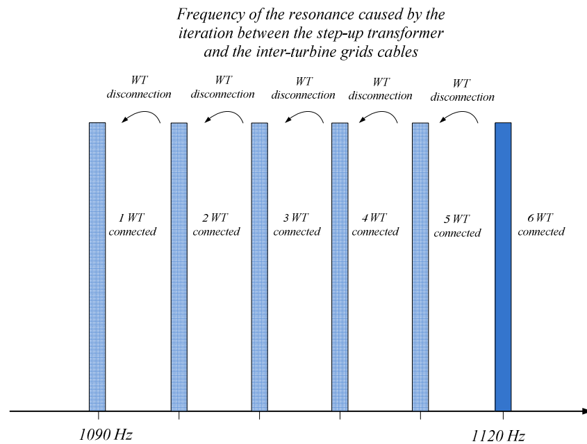
Figure 7-17: Frequency of the resonance caused by the iteration between the step-up transformer and the inter turbine cables depending on the number wind turbines connected to the feeder.
