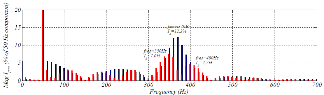
Figure 6-20: Harmonic currents at the PCC. With 2 feeders F1-F2 (red) and with 2 feeders on each primary winding F1'-F2' (black).
