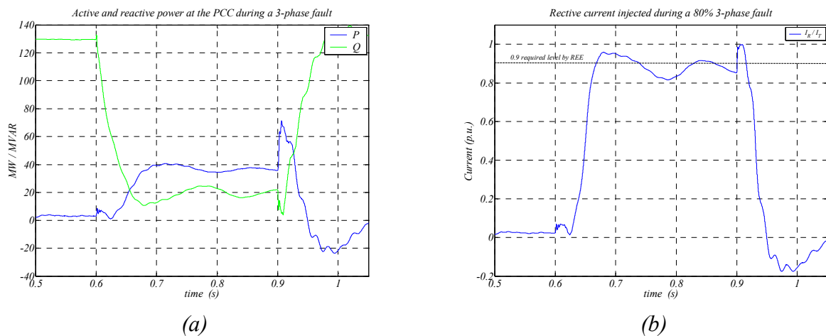
Figure 7-31: Active and reactive power at the PCC (a) and Ireactive / Itotal at the PCC (b) for the considered offshore wind farm with modified Ireactive / Itotal curve.
