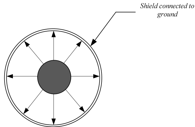
Figure 4-9: Equipotential lines of the conductor's electric field when the transmission line is provided with a shield.
