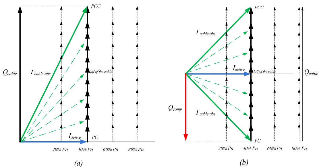
Figure 4-36: Representation of the current through the transmission line for two ways of the reactive power management: (a) reactive power compensation at one end and (b) reactive power compensation in both ends.
