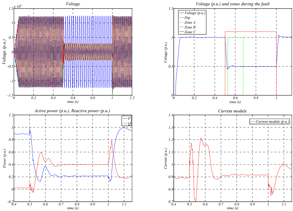
Figure 7-38: Summarized graphical results of a 4 th category fault for the test defined in the PVVC, voltage (module and signals), power and current results..
