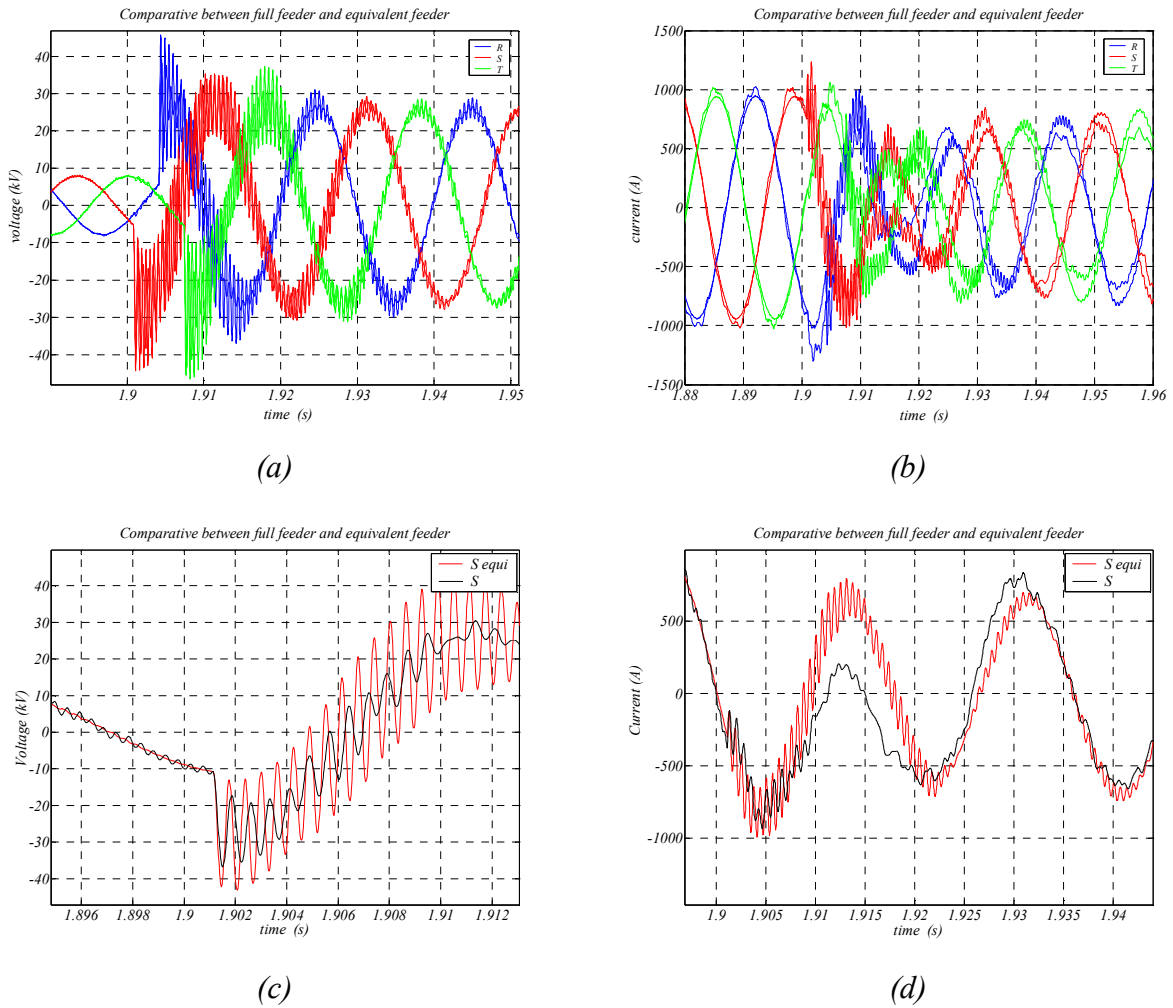
Figure F-6: Comparison of the equivalent wind turbine and the full feeder for a three-phase fault, the voltage (a) and current (b) at the PCC when the clearance of the fault occurs. (c)-(d) the voltage and current at the clearance of the fault mono-phase and more detailed, (red, equivalent feeder).
