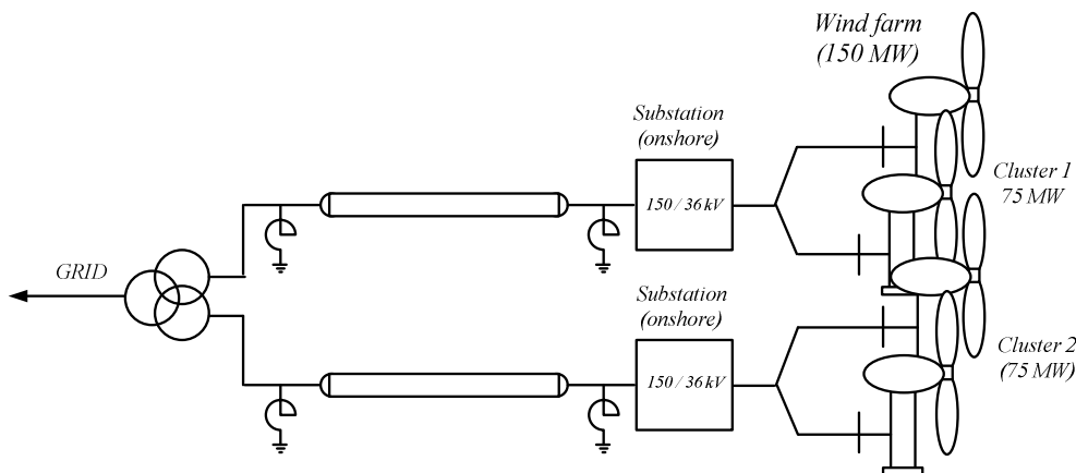
Figure 5-2: Electric configuration of a 2x75MW-150kV wind farm.
