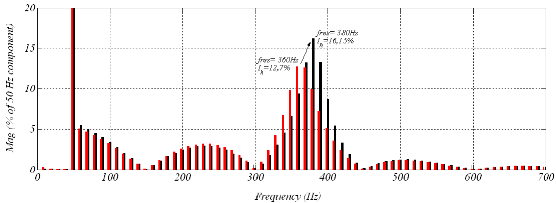
Figure 6-15: Harmonic currents at the PCC depending on the location of the harmonic voltage source inside the inter turbine grid. Substituting the 30 th wind turbine (red) and substituting the 25 th wind turbine (black).
