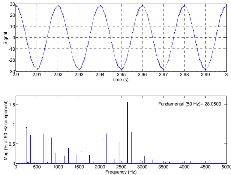
Figure 6-24: Voltage behind the connection filter of the grid side inverter and its frequency spectrum, while the equivalent wind turbine is generating the nominal power.
