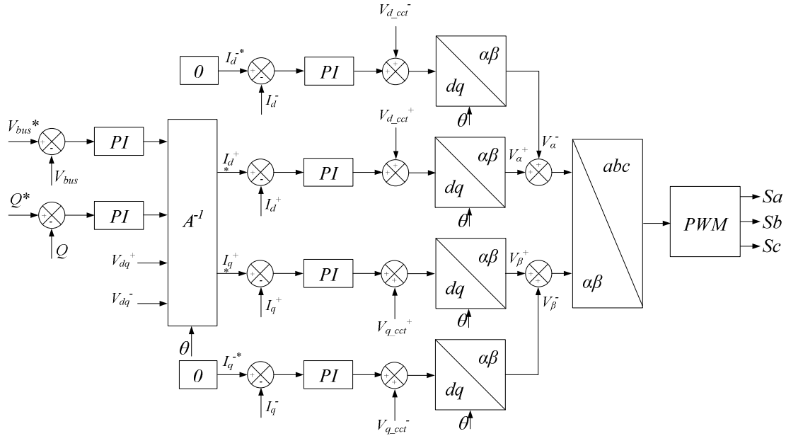
Figure 5-14: The block diagram of the implemented control strategy.
