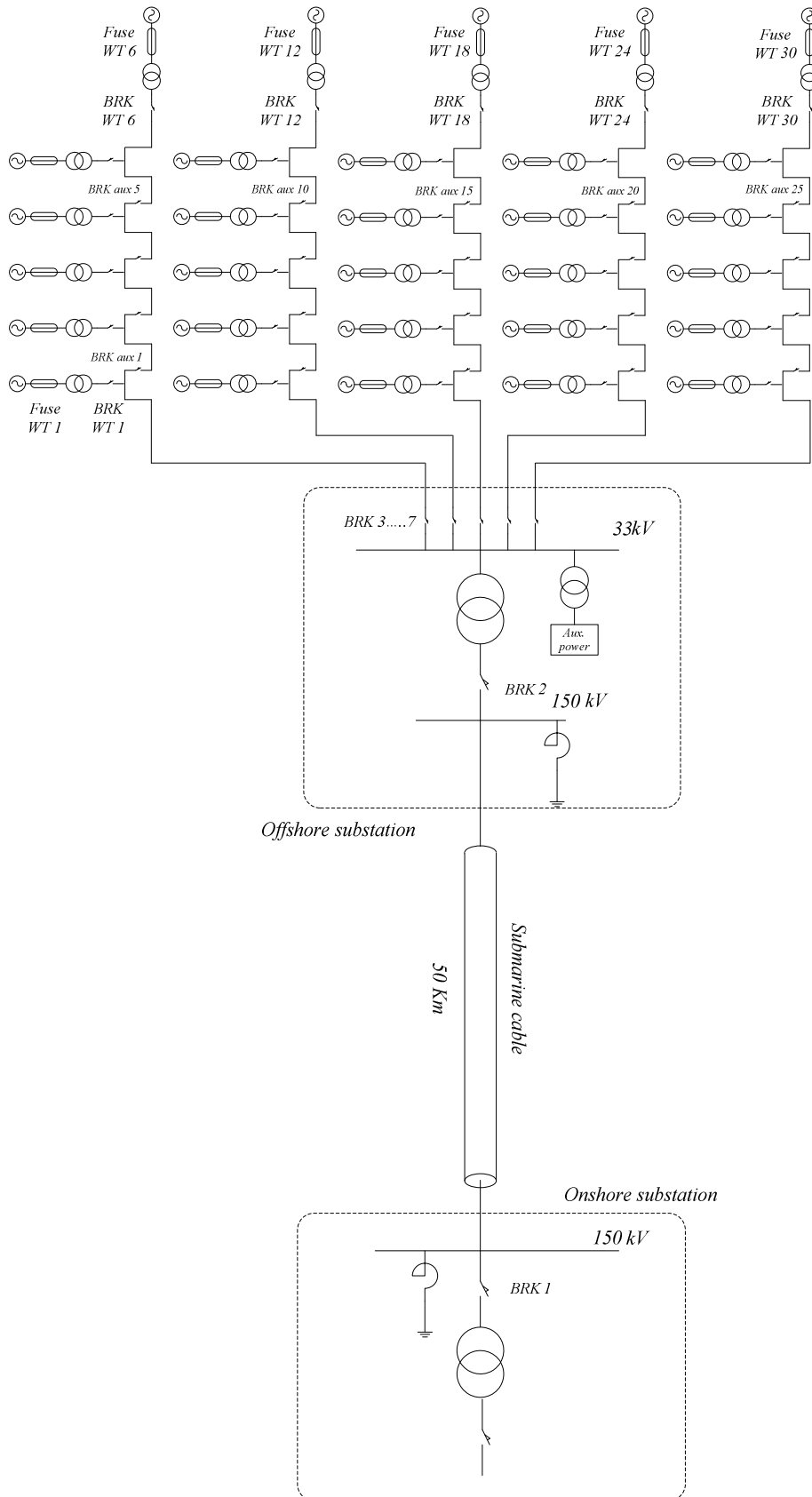
Figure 5-25: Complete electrical scheme of the considered offshore wind farm.
