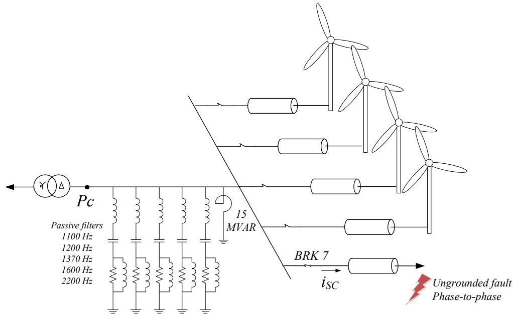
Figure 7-18: The scheme of the simulation scenario to evaluate the effect of the disconnection of a feeder during a short circuit fault.
