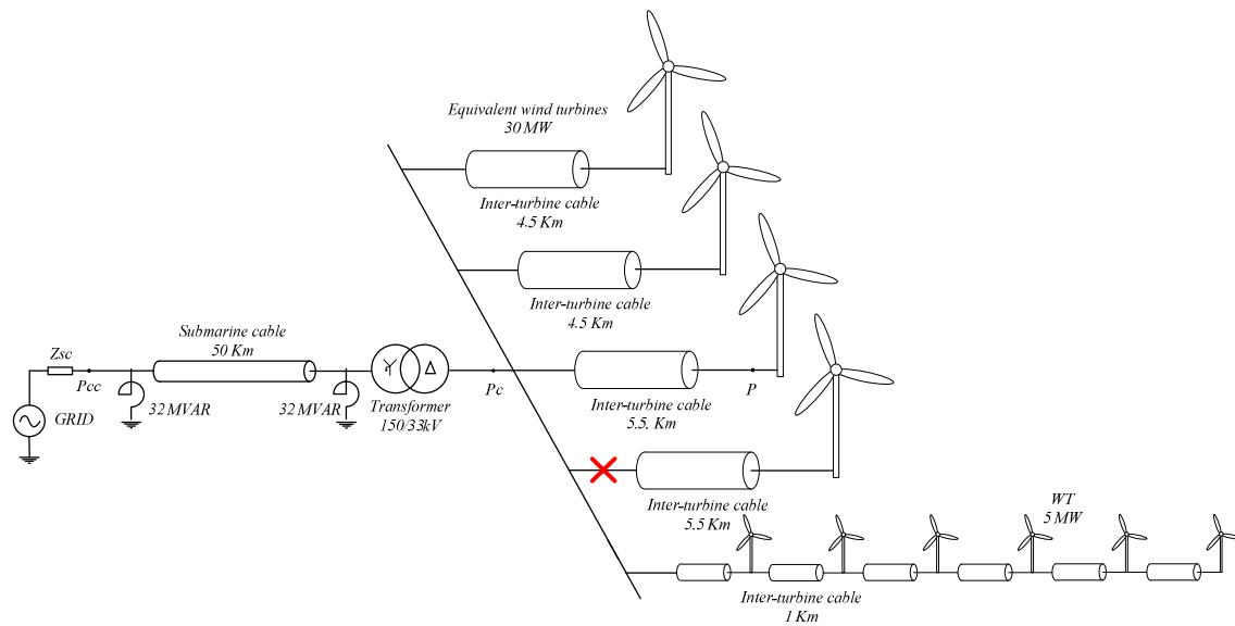
Figure 7-11: The scheme of the simulation scenario to evaluate the effect of the disconnection of a feeder.
