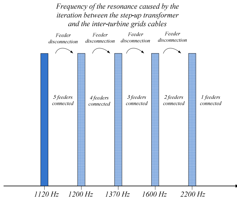
Figure 7-16: Frequency of the resonance caused by the iteration between the step-up transformer and the inter turbine cables depending on the number of feeders connected to the PC.
