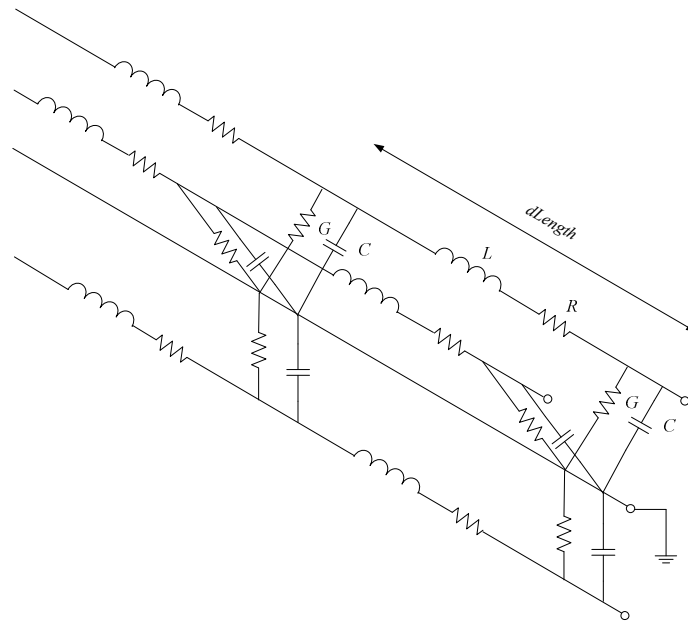
Figure 4-12: Electric representation of the three phase cable per differential length.
