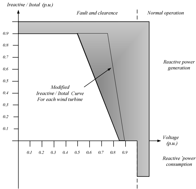
Figure 7-30: Modified Ireactive / Itotal curve depending on the voltage to fulfill the REE requirements at the PCC.
