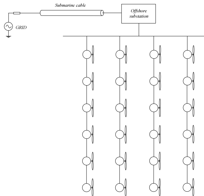
Figure 3-7: Layout of the radial design for local inter-turbine grid.
