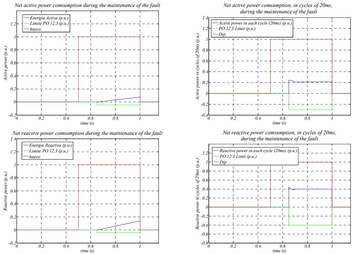
Figure 7-39: Summarized graphical results of a 4 th category fault for the test defined in the PVVC, active and reactive power consumption in B zone.
