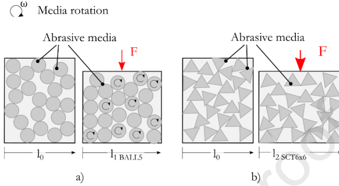
Figure 10. Illustration of the interlocking effect of abrasive media. Both medias are subjected to the same force ( F ). a) Spherical media have facility to rotate whereas b) pyramidal media do not rotate due to their angular shape.
