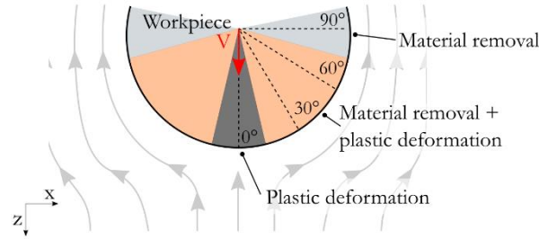
Figure 22. Interaction mechanisms during drag finishing. Plastic deformation and material removal mode regions as a function of surface orientation angle ( \alpha ) regarding media flow (grey arrows).
