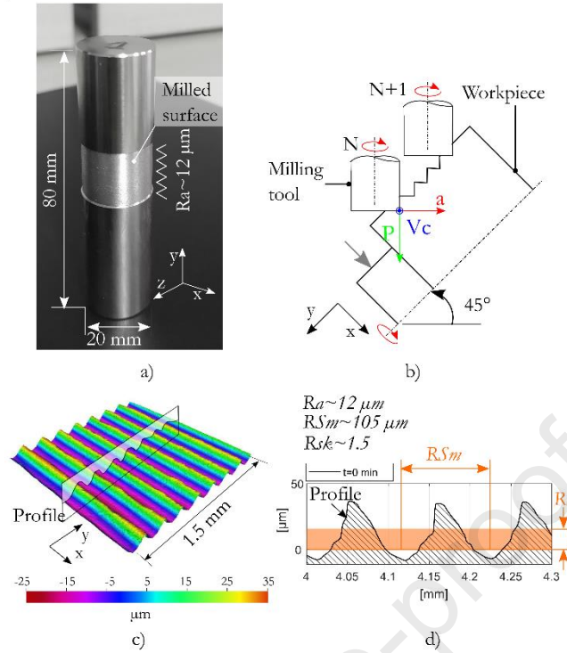
Figure 17. Sample fabrication and characteristics. a) Sample shape and dimensions with a milled surface of Ra=12 \mu m , b) milling process used to create the periodical surface, c) the details of the periodical surface in 3D, and d) its surface profile in 2D and Ra , RSm and Rsk values.
