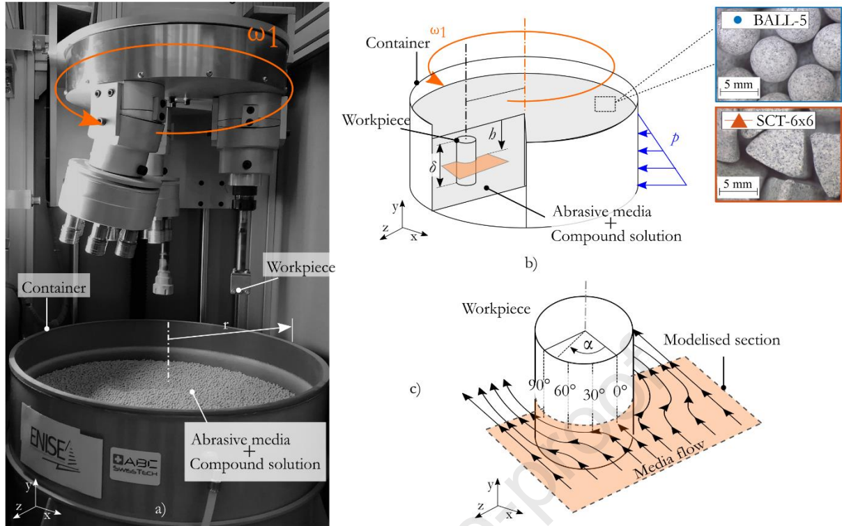
Figure 2. The experimental set-up. a) The drag finishing machine and the motion applied to the system ( \omega_1 ), b) the schematic drawing of the set-up indicating the rotational speed ( \omega_1 ), the immersion depth ( b ), the height of the part ( \delta ) and the hydrostatic pressure ( p ). And in c) the interaction between the part and media flow. The analysed orientation angles ( \alpha ) (0, 30, 60, 90°) were indicated in c) as well as the modelled section.
