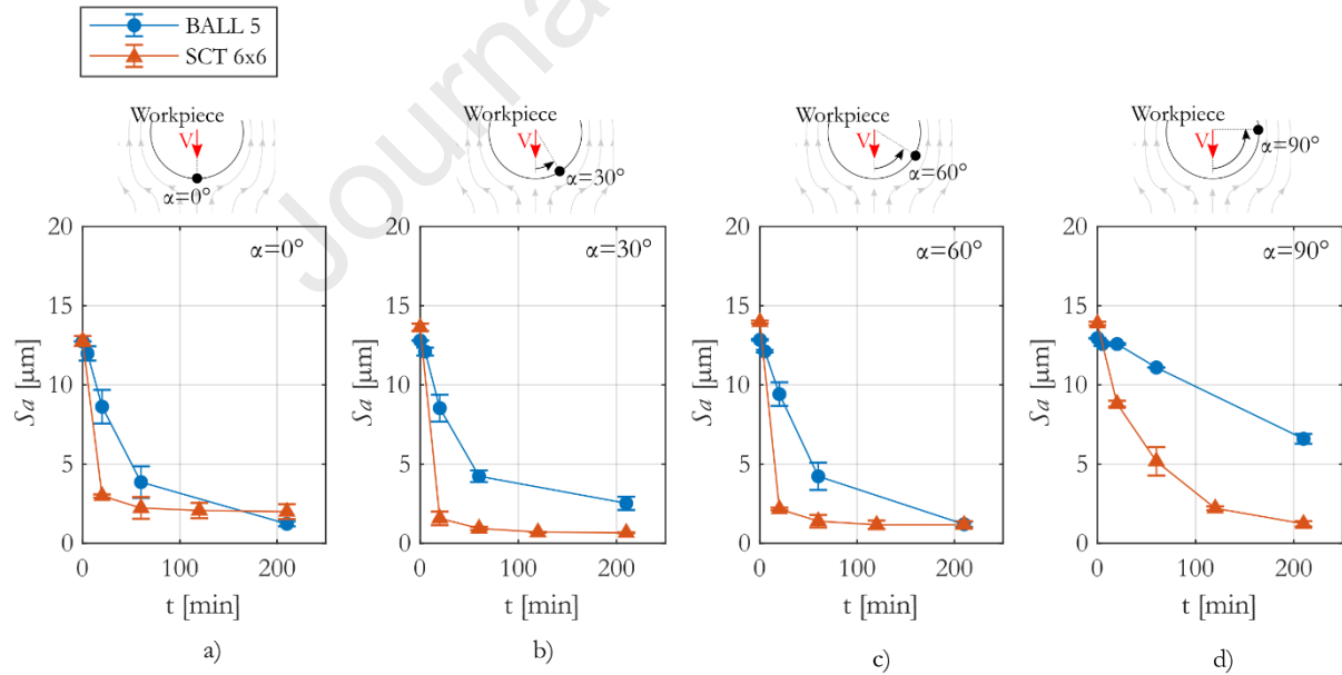
Figure 19. S_a evolution graphs. S_a after 210 min of drag finishing for both abrasive media (BALL5 and SCT 6x6) at four surface orientations ( \alpha ) a) 0^\circ , b) 30^\circ , c) 60^\circ and d) 90^\circ .
