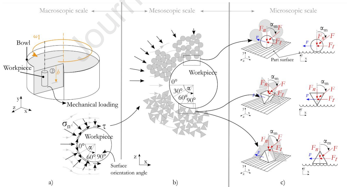
Figure 1. Drag finishing, a multiscale process. Drag finishing process at a) a macroscopic scale considering media as an abrasive slurry and the resultant mechanical loadings (normal and shear stresses, \sigma_n et \tau ) at the interface. b) At a mesoscopic scale, where the mixture of abrasive media (discrete particles) interacts with the part to polish. c) Finally, at a microscopic scale single abrasive particles interact with the surface roughness under different contact forces ( F_n , F_t , F ), sliding velocities ( v ) and orientation angles ( \alpha_m ).
