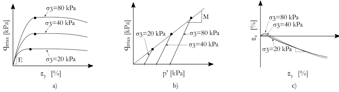
Figure 7. The typical representation of triaxial test results: a) deviatoric stress ( q_{triax} ) vs. the vertical strain ( \epsilon_y ), b) deviatoric stress ( q_{triax} ) vs. the effective mean stress ( p' ) and c) radial strain ( \epsilon_v ) vs. vertical strain ( \epsilon_y ). All tests are made at three confining pressures ( \sigma_3 ), 20, 40 and 80 kPa. From these graphs, the identification of the Young's Modulus ( E ), the Poisson's ratio ( \nu ), the friction angle ( \varphi ) and the dilatancy angle ( \psi ) is calculated.
