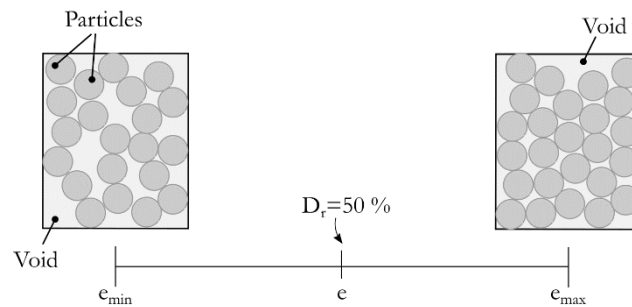
Figure 6. The various compaction levels of granular materials, maximum and minimum void ratios ( e_{min} and e_{max} ) and the void ratio ( e ) for a relative density D_r of 50%.
