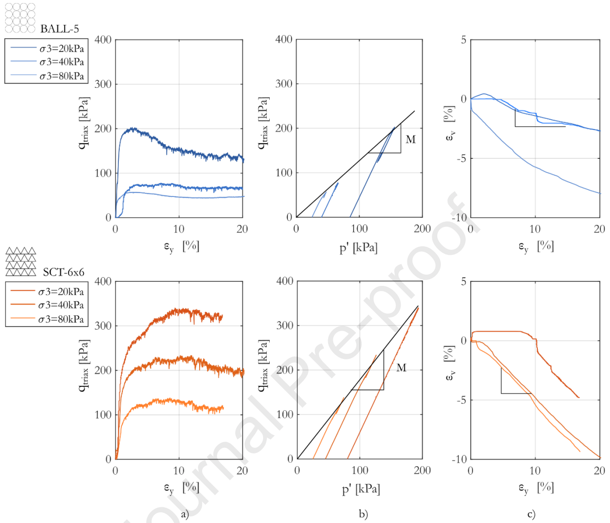
Figure 9. Triaxial test results for both media. a) deviatoric stress ( q_{\text{triax}} ) vs. the vertical strain ( \epsilon_y ), b) deviatoric stress ( q_{\text{triax}} ) vs. the effective mean stress ( p' ) and c) radial strain ( \epsilon_v ) vs. vertical strain ( \epsilon_y ) for both medias at different confining stresses ( \sigma_3 ): 20, 40, 80 kPa.
