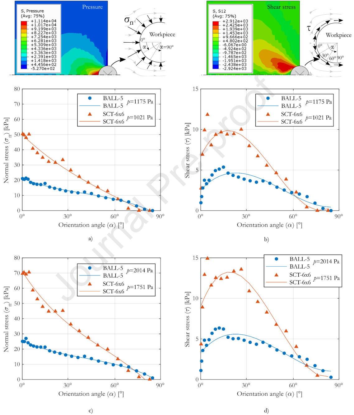
Figure 16. The numerical mechanical loading. a) Normal stress ( \sigma_n ) and b) shear stress ( \tau ) distribution around the part for two hydrostatic pressures ( p ) and two immersion depths ( h ) for spherical and pyramidal medias.
