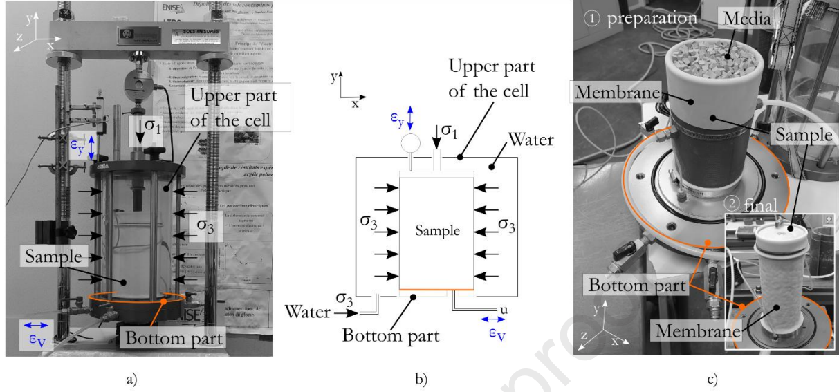
Figure 5. The triaxial tests for media characterisation. a) The employed triaxial cell and its b) schematic illustration where the sample, the applied stresses ( \sigma_1, \sigma_3 ) and the deformation sensors ( \epsilon_y, \epsilon_v ) are shown. In c), sample preparation is shown: 1) abrasive media embedded in the deformable membrane and 2) the closed sample is also shown.
