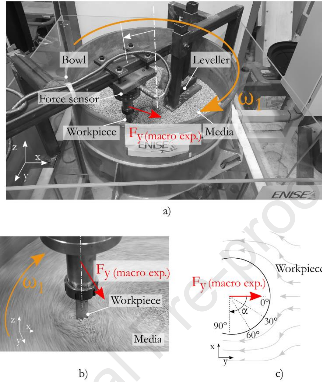
Figure 12. The experimental set-up for drag force measurements. a) Developed experimental set-up to measure the macroscopical experimental drag forces ( F_y(\text{macro exp.}) ). The components: the bowl or container, the leveller, the media, workpiece and the force sensor are indicated. The container rotates around its own axis with a rotational speed \omega_1 . In b), a zoom of the media flow around the part is shown and in c) a schematic explanation is shown, indicating media flow and the drag force.
