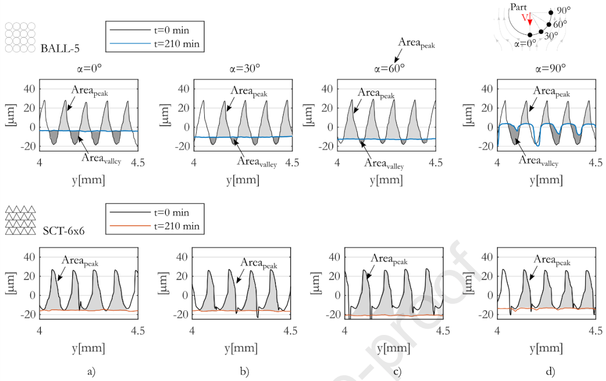
Figure 20. Initial and final (t=210 min) primary profiles. For surfaces polished with BALL-5 and SCT 6x6 at four surface orientations (α): a) 0°, b) 30°, c) 60° and d) 90°. Peak and valley areas are indicated in grey colours (Area peak and Area valley ).
