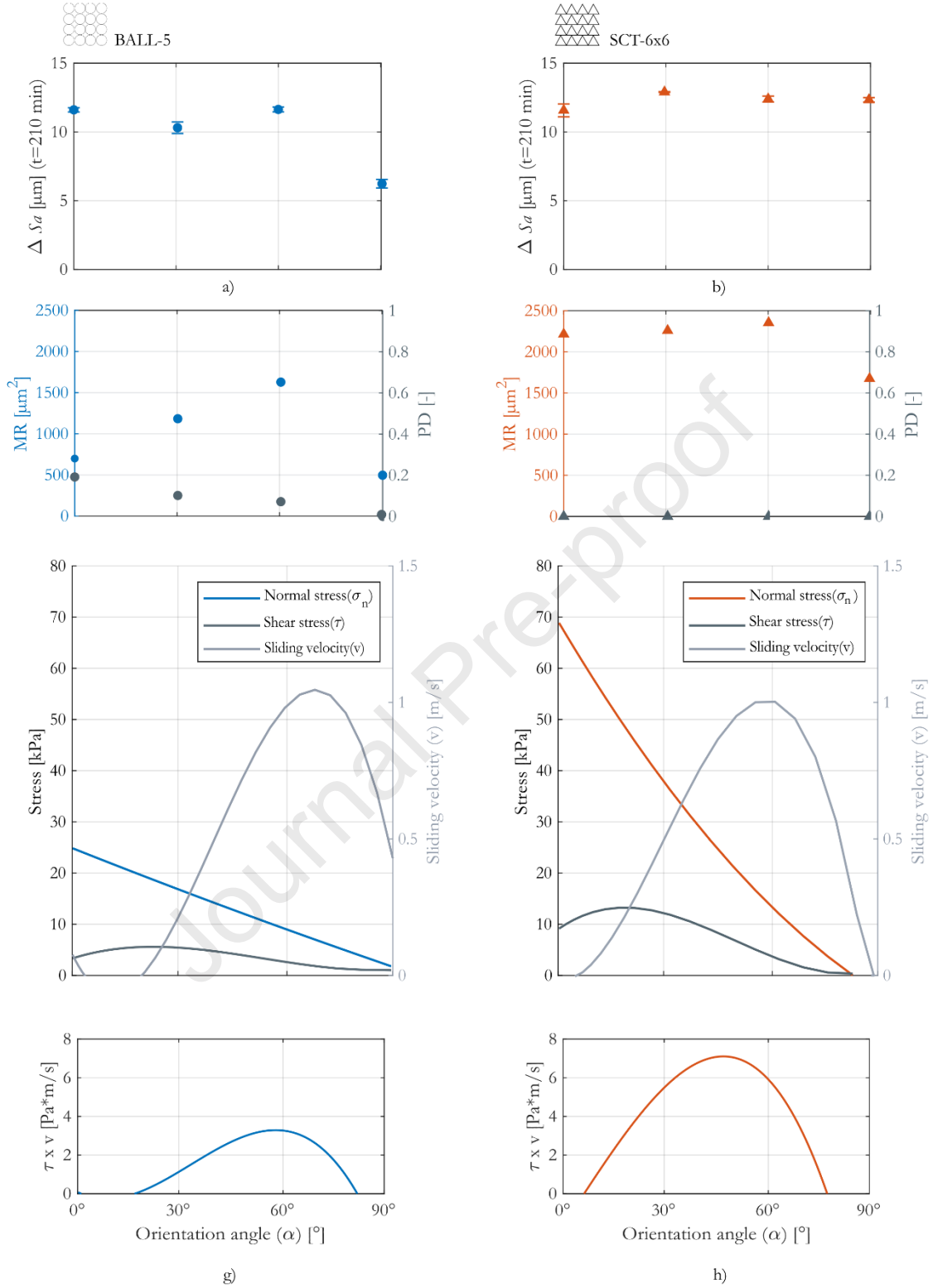
Figure 21. Correlation between experimental and numerical results. Experimental surface roughness difference ( \Delta Sa ) depending on the orientation angle ( \alpha ) for a) spherical and b) pyramidal medias. Material removal and plastic deformation mechanisms for each orientation angle and each abrasive media: c) spherical and d) pyramidal medias. In e), f), the numerical mechanical loading (sliding velocity, v , normal \sigma_n and shear stresses \tau ) are shown for both abrasive medias. Finally, in g) and h), the shearing energy is calculated to show the optimal orientation angle.
