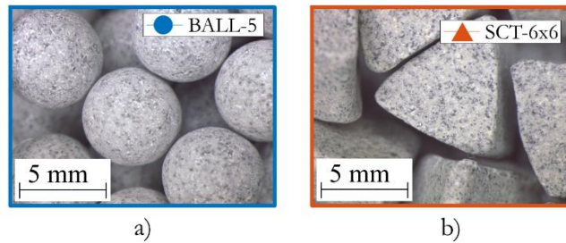
Figure 8. Ceramic abrasive media of different shape: a) spherical, \varnothing=5 mm, and b) pyramidal, dimensions=6x6 mm. Both medias had the same composition and were provided by ABCSwissTech.
