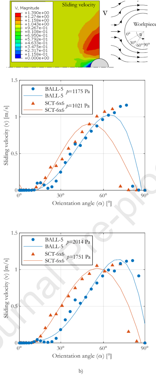
Figure 15. Media sliding velocity distribution around the part ( v ) for two pressures ( p ) and two immersion depths ( b ) for spherical and pyramidal medias.
